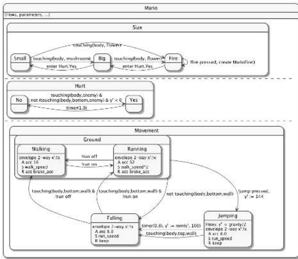
Figure 3: (Simplified) Super Mario as a hybrid automaton.
