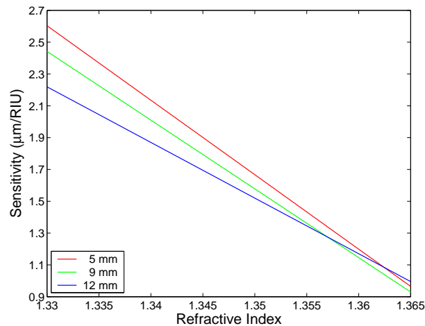
FIG. 7 The sensitivity as a function of the refractive index of the aqueous solution of ethanol for three lengths of the sensitive region of the fibre.
