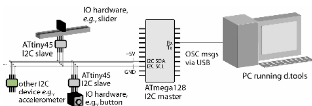
Figure 6. The d.tools architecture uses standardized, open protocols for hardware and PC communication.
