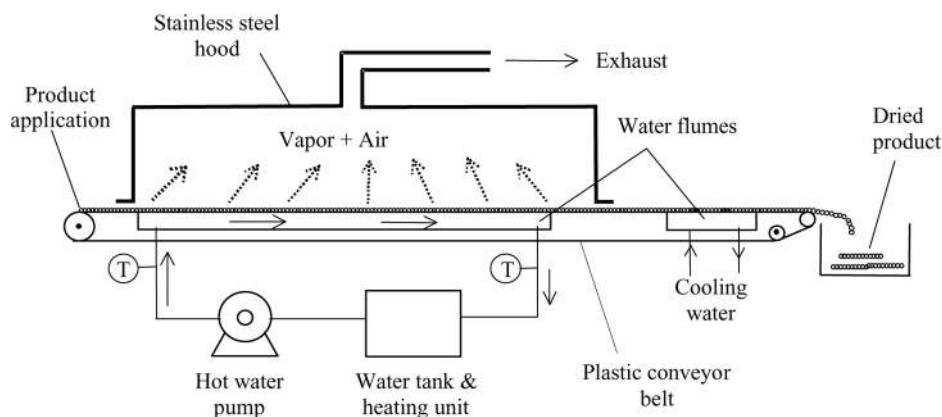
FIG. 2. Schematic diagram of Refractance Window ® drying system (from Nindo et al. [47] ).
