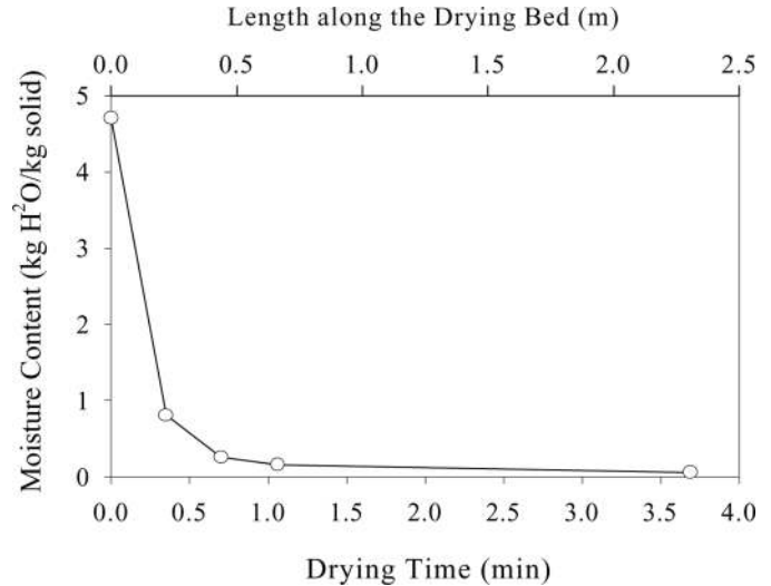
FIG. 4. Typical product residence time during RW drying of strawberry puree using process water temperature at 95°C and puree thickness of about 1.0 mm (From Ref. 46).
