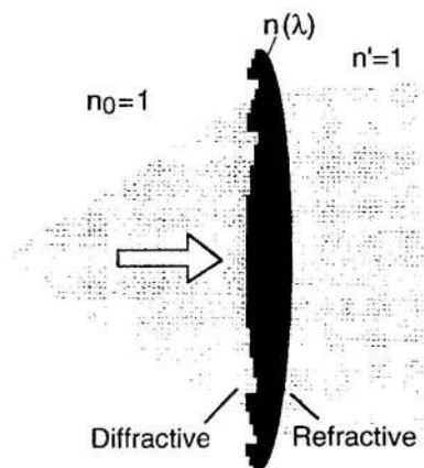
Fig. 7. Hybrid (refractive-diffractive) lens.
