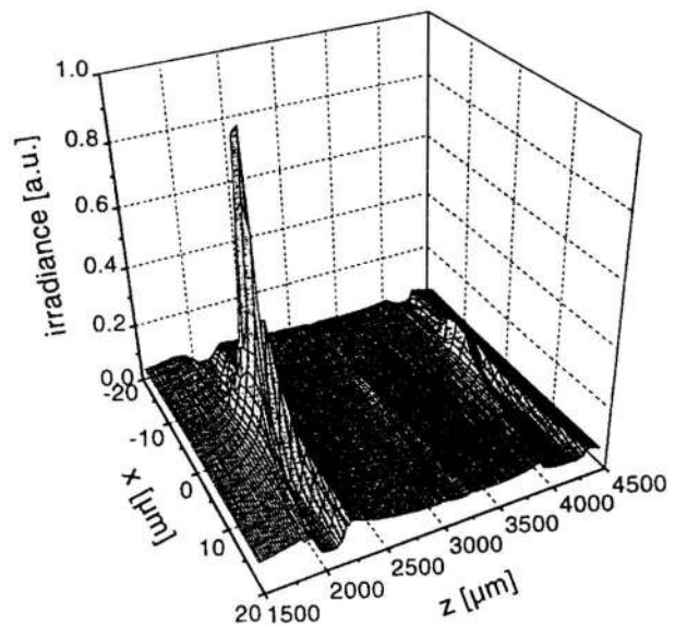
Fig. 9. Measured irradiance distribution in the image space of an f/1 PMFE.
