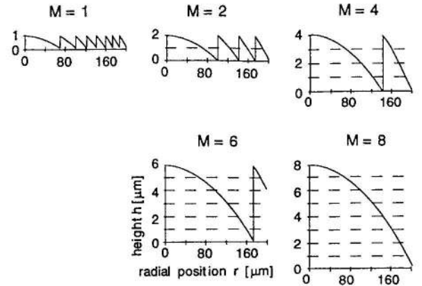
Fig. 4. PMFE surface-relief elements for numerical simulations.
