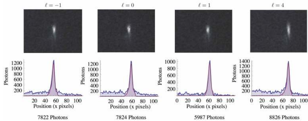
Fig. 4. Using a EMCCD camera in single photon counting mode, images were generated by summing over 16383 frames. Each pixel has a dark count rate, generating noise in every pixels in the camera. The images shown are the raw captured images. The dark count rate was assessed by counting the photons over the same capture period with the camera shutter closed. A threshold was set with a value corresponding to the mean, plus one standard deviation of the dark count rate. The corresponding graph is a sum of each column, in blue, and superimposed with the results when a Wiener Noise reduction filter is applied shown in red. Summing under the red curve gives us an approximation of the number of photons received at the camera plane.
