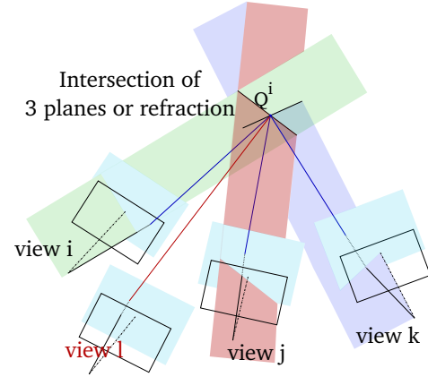
Figure 5. Four-view refractive geometry relationship. Considering the intersection of three planes of refraction i, j and k defined by the light rays corresponding to the 3D point Q^i and the camera's axis, we refine estimates of the fourth view camera pose by ensuring light ray l to pass through Q^i .
