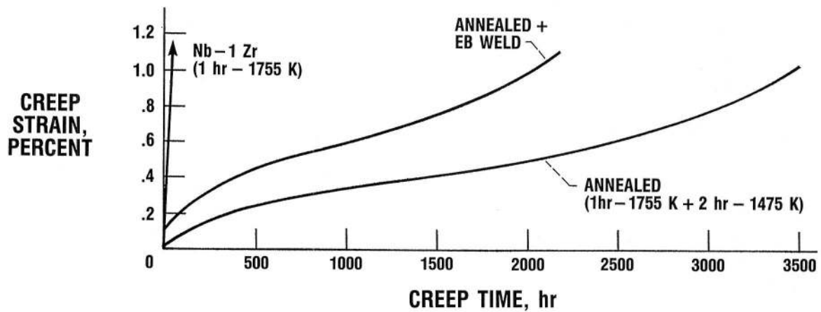
FIGURE 7. - CREEP CURVES OF Nb-1Zr AND PWC-11 AT 1350 K AND 40 MPa.
