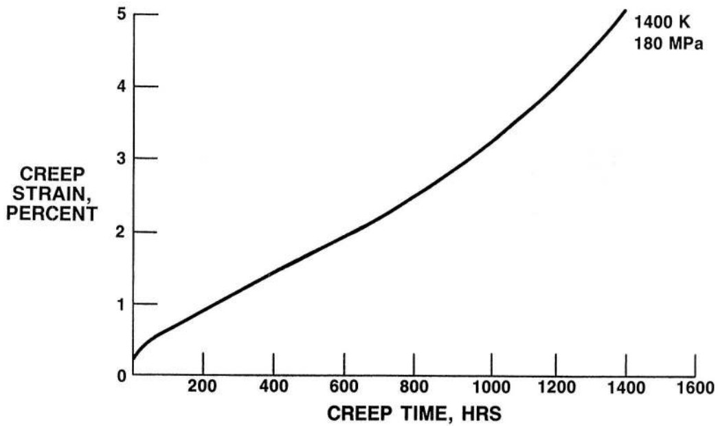
FIGURE 19. - TYPICAL CREEP CURVE FOR ST300/Nb + 1Zr COMPOSITE.
