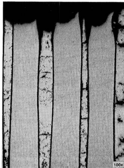
FIGURE 21. - FRACTURE SECTION OF ST300/Nb + 12r CREEP RUPTURE SPECIMEN.
