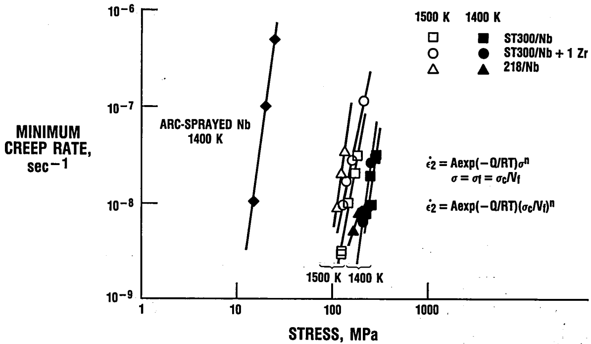
FIGURE 24. - COMPARISON OF MINIMUM CREEP RATE FOR COMPOSITES.
