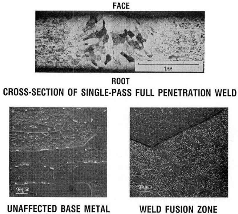
FIGURE 6. - MICROSTRUCTURES OF ELECTRON BEAM WELDED PWC-11.
