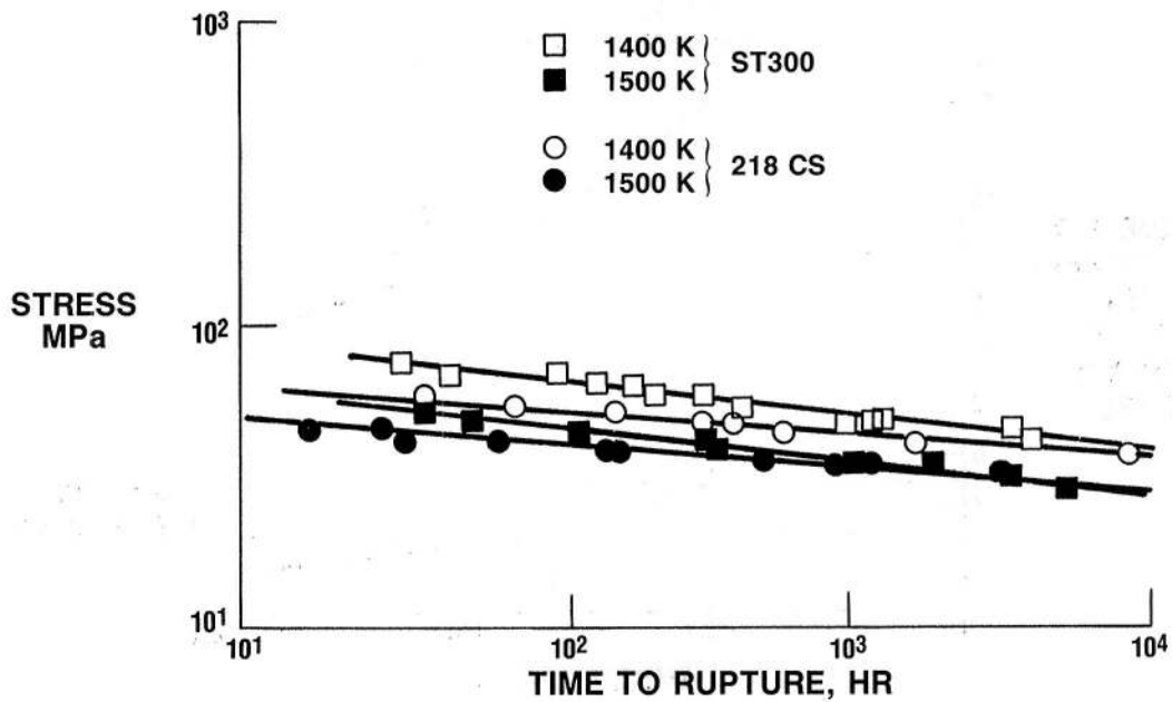
FIGURE 11. - STRESS RUPTURE STRENGTH FOR ST300 (W + 1.5% ThO 2 ) AND 218 CS FIBERS.
