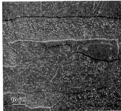
PWC-11 ANNEALED 1 HR-1755 K + 2 HRS-1475 K
