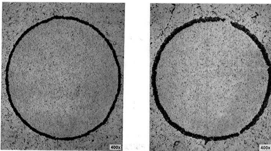
FIGURE 15. - ST300/Nb + 1Zr FIBER/MATRIX REACTION.
