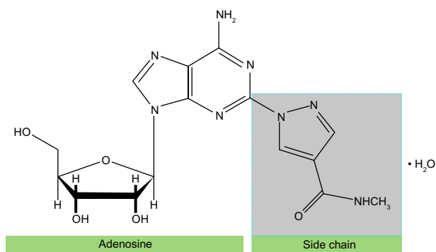
Figure 2 Regadenoson molecule.
