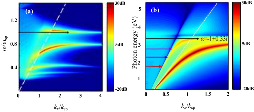
Fig. 1. Computed isotherm contour of transmissivity |T_p|^2 of (a) a conceptual NRIM slab and (b) a 50-nm silver film surrounded by air and glass ( n = 1.52 ). In (a) d = 0.14\lambda_{sp} ; \varepsilon_2 = 1 - 2\omega_{sp}^2/(\omega^2 + 0.01i\omega\omega_{sp}) , and \mu_2 = 1 - 1.6\omega_{sp}^2/[(\omega - 0.106\omega_{sp})^2 + 0.01i\omega\omega_{sp}] , k_{sp} = \omega_{sp}/c . In (b) the permittivity data are taken from Ref. [7].
