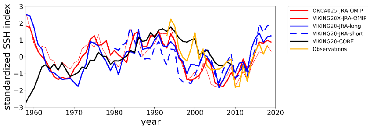
Figure 10. Time series of the annual mean subpolar gyre index in the experiments and based on observations (orange). Here, the index is defined as the second PC of an EOF-analysis for non-detrended SSH in the North Atlantic between 20 and 70°N.
