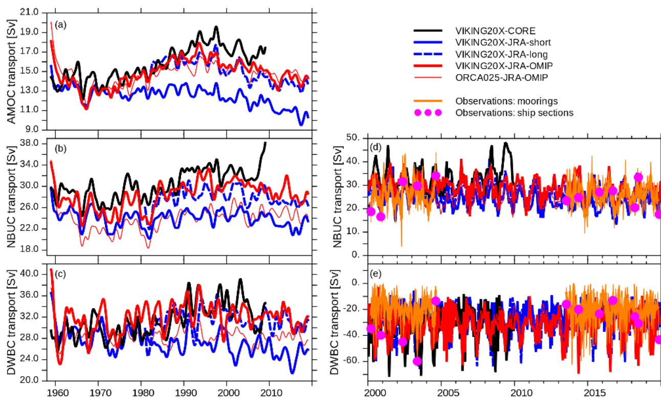
Figure 17. Time series of interannually filtered (a) AMOC, (b) NBUC and (c) DWBC transports at 11^{\circ}\text{S} ; monthly averages of positive (NNE-ward) NBUC and negative (SSW-ward) DWBC transports (see Table 7 for details of the definitions) are given in (d) and (e) together with mooring based (orange curves; thick monthly, thin 2.5-day averages) and ship based observations (purple dots)
