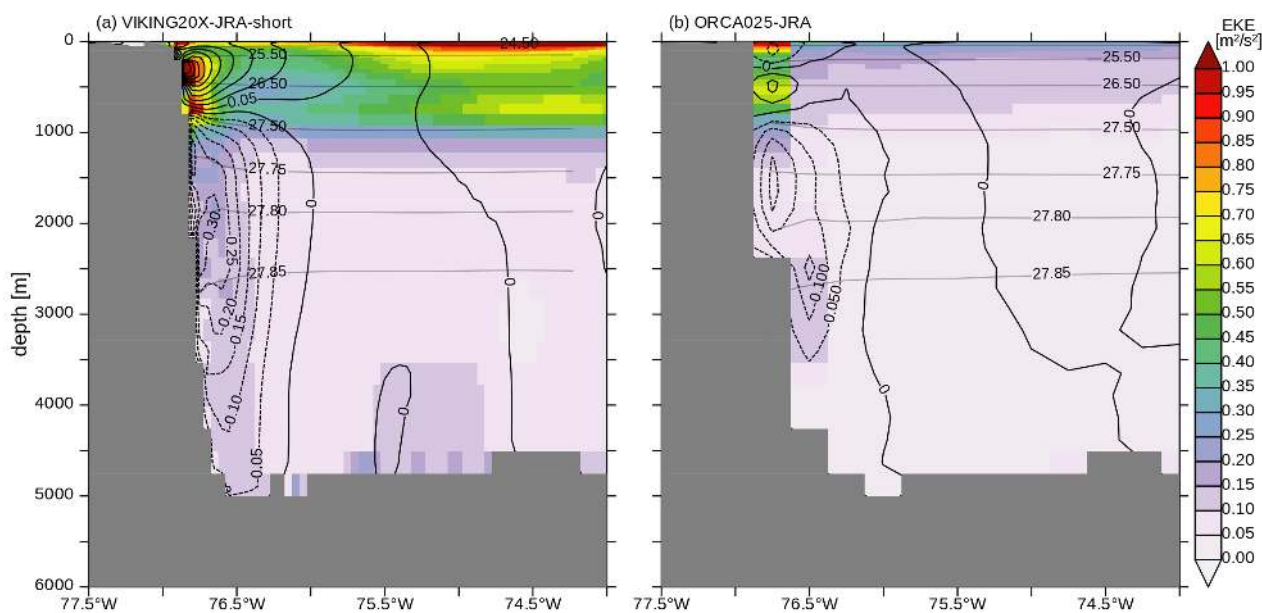
Figure 13. Mean (1990-2009) EKE in \text{m}^2 \text{s}^{-2} (shaded) and meridional velocity (black contours) section at 26.5^\circ\text{N} for (a) VIKING20X-JRA-short and (b) ORCA025-JRA with \sigma_0 isolines (grey).
