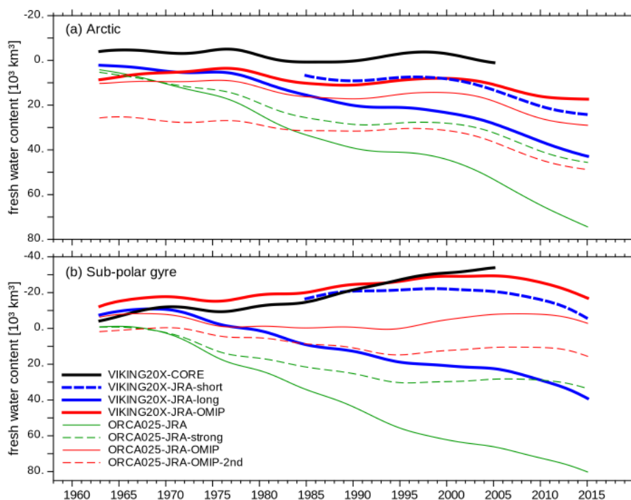
Figure 6. Pentadally filtered (a) Arctic and (b) subpolar Freshwater Content (computed from seawater alone, hence excluding sea-ice and snow volume, using a reference salinity of S_{ref} = 34.7 , in 10^3 \text{ km}^3 ). Note the inverted y-axis.
