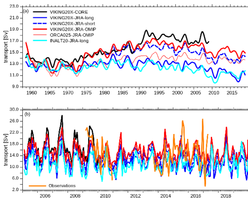
Figure 19. Time series of the AMOC strength at 34.5°S (a) interannually filtered and (b) monthly averages for the most recent 15 years with observations from Meinen et al. (2018) (orange).
