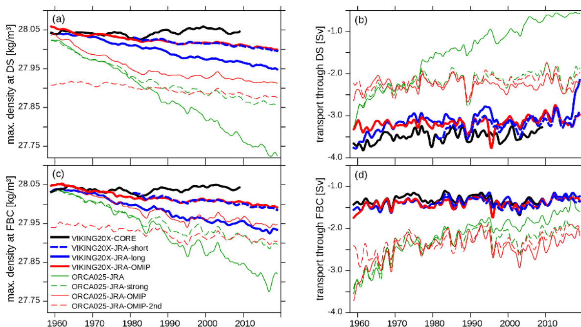
Figure 8. Evolution of maximum overflow density and the overflow transport in the (a and b) Denmark Strait and the (c and d) Faroe-Bank Channel respectively. Overflow transport estimates are based on southward transport of waters with density larger than 27.70 \text{ kg m}^{-3} below 270 m.
