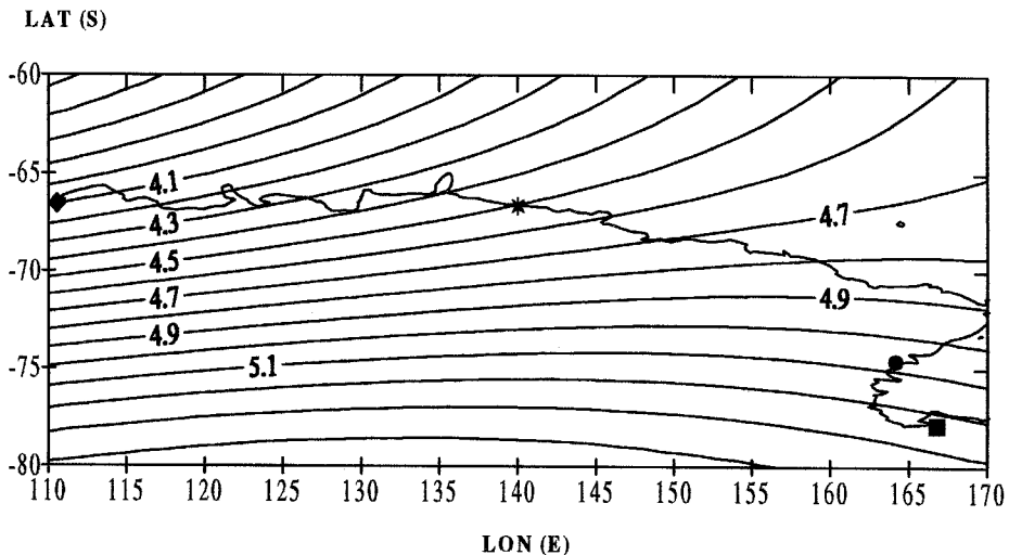
Fig. 1. Regional monthly median map of f_0F_2 obtained by SIRM for December 1993 ( R_{12} = 40 ) at 00UT. The ionospheric stations used for calculating the SIRM coefficients are: ♦ Casey (66.3S, 110.5E), * Terre Adelie (66.7S, 140.0E), and ■ Scott Base (77.9S, 166.8E). f_0F_2 monthly medians from ● Terra Nova Bay (74.70S, 164.12E), not included in the database for the SIRM coefficients evaluation, are used for comparison with SIRM modelled values.
