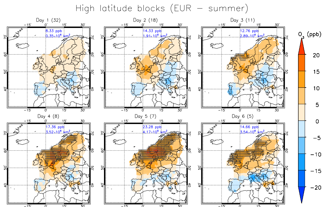
Figure 6. Evolution of MDA8 O_3 anomalies under the influence of EUR blocking in summer. The panels show, from left to right and from top to bottom, the average anomalies on the first six days a block is in the sector. The total number of blocks considered is given in brackets on the top of each panel. The maximum anomaly found (ppb) and the total area with anomalies higher than 5 ppb ( \text{km}^2 ) are also indicated in blue colour. Grey open squares indicate grid cells where the ozone composite under blocking exceeds the 90th percentile of the summer distribution.
