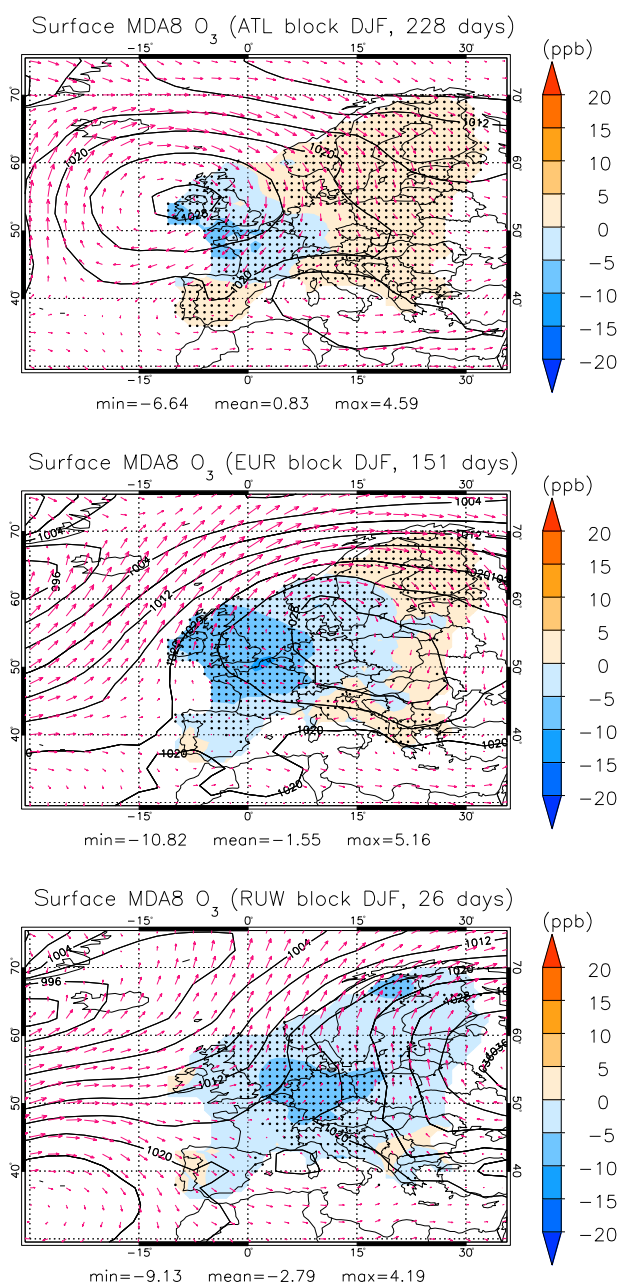
Figure 10. As Fig. 4 but for blocking centres remaining in the Atlantic ( 30\text{--}0^\circ\text{W} , top) and European ( 0\text{--}30^\circ\text{E} , middle) sectors as well as in the west flank of the Russian sector ( 30\text{--}45^\circ\text{E} , bottom) in winter.
