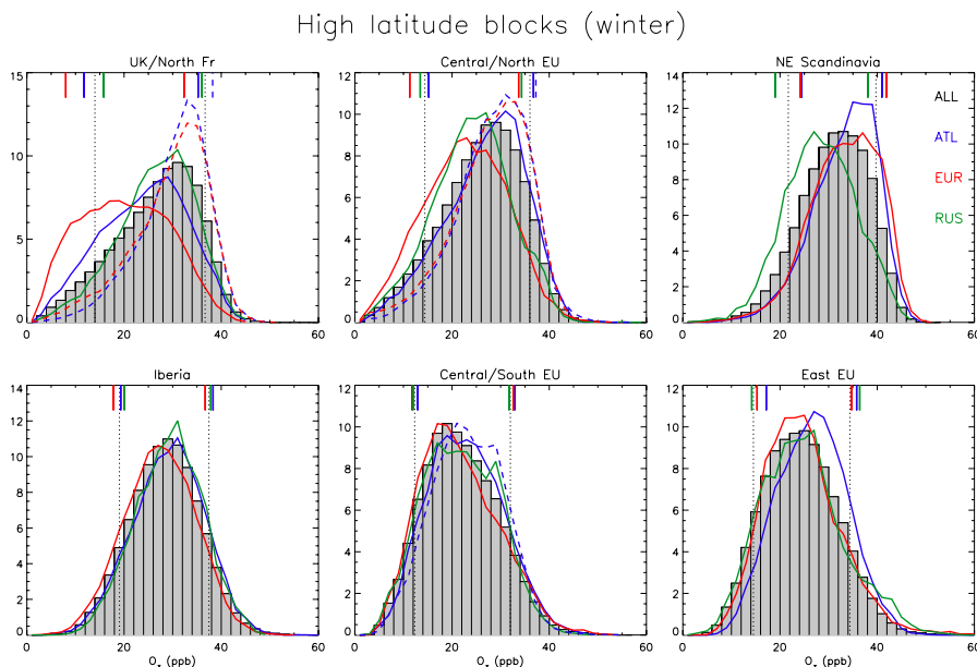
Figure 11. As Fig. 5 but for winter blocking. Note that blue and red dashed lines have been added to represent the frequency distributions of the data within the “UK/North Fr” and “Central/North EU” boxes when ridge centres are located over the ATL and EUR sectors, respectively. Data on days with ATL ridges are also shown for the “Central/South EU” region.
