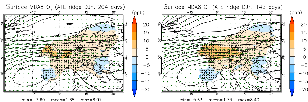
Figure 12. As Fig. 4 but for subtropical ridge centres in the Atlantic ( 30\text{--}0^\circ W, left) and east Atlantic ( 15\text{--}0^\circ W, right) in winter.
