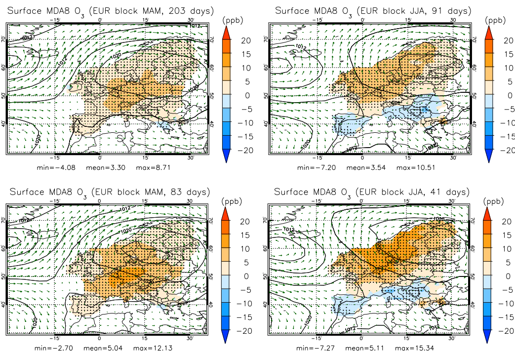
Figure 4. Composites of the seasonal anomalies of surface MDA8 O 3 (ppb) for days with blocking centres over the European sector (EUR, 0–30° E) during spring (left) and summer (right). Anomalies have been calculated with respect to the MDA8 O 3 mixing ratios on days without EUR blocking in that season during the 1998–2012 period. All data on days with blocking centres remaining over 0–30° E (top) and data only from the third day with blocks in that sector (bottom) have been taken into account for the calculation of the ozone anomalies. Stippling indicates statistically significant anomalies at the 5% level (two-sided t test). The black contour lines depict the composites of MSLP (hPa) for those days. Horizontal wind fields at 850 hPa are displayed by arrows. The total number of days considered is indicated on the top of each panel.
