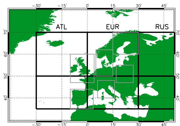
Figure 2. Longitudinal sectors considered for the identification of the centres of high-latitude blocks (northern black boxes) and subtropical ridges (southern black boxes): Atlantic (ATL, 30–0° W), European (EUR, 0–30° E) and Russian (RUS, 30–60° E, only partially shown). Grey boxes identify the geographic areas considered in the regional assessment performed in Sects. 3 and 4. The regions considered, from west to east and from north to south, are “UK/North Fr”, “Central/North EU”, “NE Scandinavia”, “Iberia”, “Central/South EU” and “East EU”.
