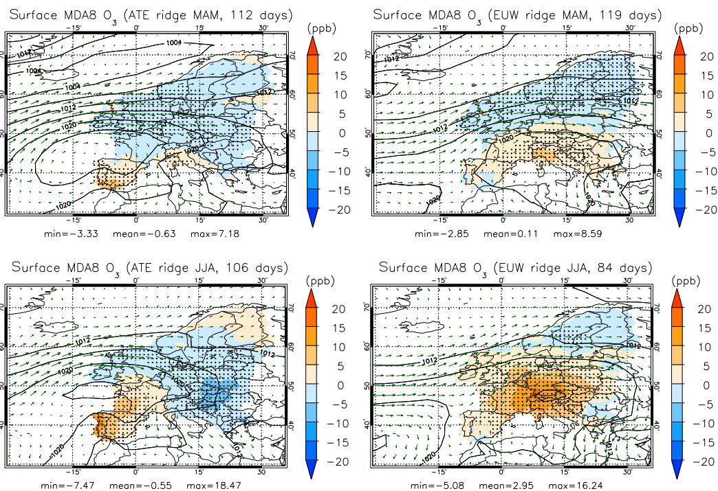
Figure 8. As Fig. 4 but for sub-tropical ridges with centres over the east Atlantic ( 15\text{--}0^\circ W, left) and the west of the EUR sector ( 0\text{--}15^\circ E, right) in spring (top) and summer (bottom).
