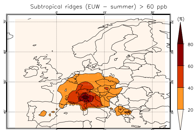
Figure 9. Percentage of summer days with ridge centres within the west flank of the EUR sector ( 0\text{--}15^\circ E) for which the 60 ppb MDA8 \text{O}_3 target is breached. Note the similar geographic location of the region with exceedances on more than 40 % of the days in this figure and that where the local 90th percentile is surpassed on more than 30 % of the days under this synoptic situation (Fig. 7, upper right).
