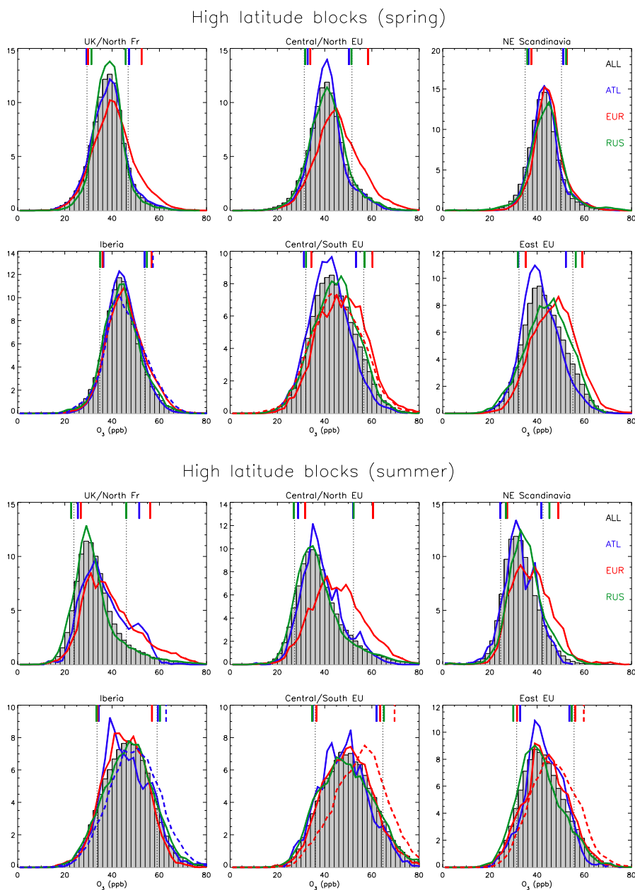
Figure 5. Spring (upper panels) and summer (lower panels) probability frequency distributions (%) of MDA8 O 3 for the six regional boxes presented in Fig. 2 under different synoptic situations. Grey bars denote the 1998–2012 seasonal climatology. Solid lines correspond to days with block centres over the Atlantic (blue), European (red) and Russian (green) sectors. Blue and red dashed lines also represent the frequency distributions of the data when ridge centres are located over the ATL and EUR sectors, respectively; they are only shown for the regions and seasons where surface ozone presents the strongest responses to ridges. The width of the bins is 2 ppb. The horizontal position of the vertical dotted lines represents the 10th and 90th percentiles of the climatology, while the short vertical lines on the top of the plots indicate the values of the 10th and 90th percentiles under the influence of ATL, EUR and RUS blocking. The 90th percentiles of the data with ridges are also displayed as dashed lines when they are above those with blocking.
