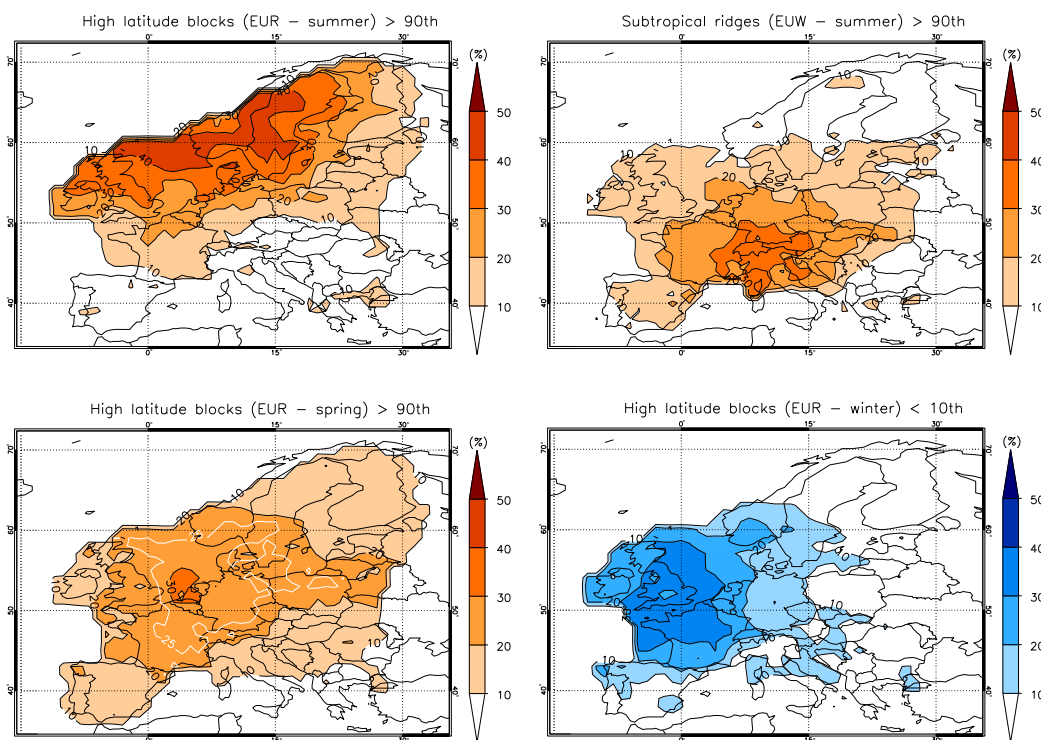
Figure 7. Percentage of EUR blocking days in summer (upper left) and spring (bottom left) as well as of days with ridges over the west of the EUR sector in summer ( 0\text{--}15^\circ\text{E} , upper right) for which MDA8 \text{O}_3 is above the local 90th percentile of its seasonal distribution. The lower right panel also shows the percentage of EUR blocking days with MDA8 \text{O}_3 below the 10th percentile of its seasonal distribution in winter.
