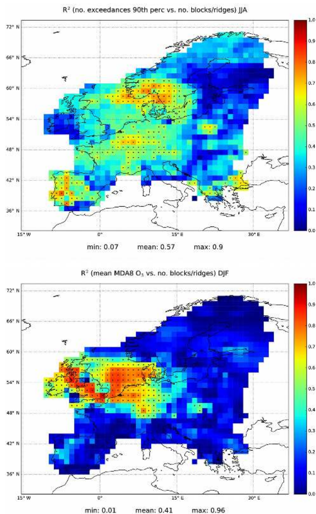
Figure 13. Coefficient of determination ( R^2 ) of two multiple linear models predicting the number of exceedances of the 90th O_3 percentile in summer (top panel, Eq. 1) and the winter mean O_3 mixing ratios (bottom panel, Eq. 2) over each grid cell as a function of the interannual variability of blocks and ridges. Stippling indicates the locations where the multiple linear fits are significant at the 5% level ( F test).
