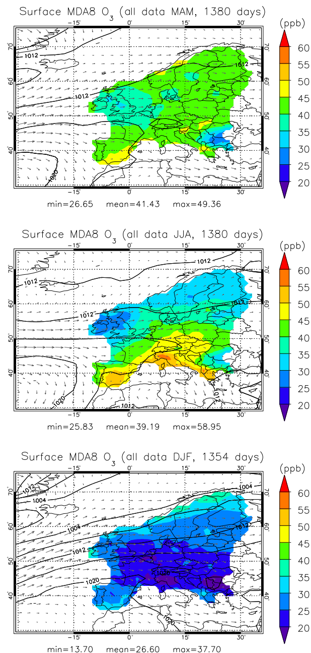
Figure 1. Composites of the seasonal means of maximum daily 8 h running average near-surface ozone (MDA8 O_3 ) expressed in parts per billion by volume (ppb, shaded areas) in spring (top), summer (middle) and winter (bottom) during the 1998–2012 period. The black contour lines depict the mean sea level pressure (MSLP) for the same period, expressed in hPa. Arrows indicate horizontal winds at 850 hPa. The total number of days considered is indicated on the top of each panel.
