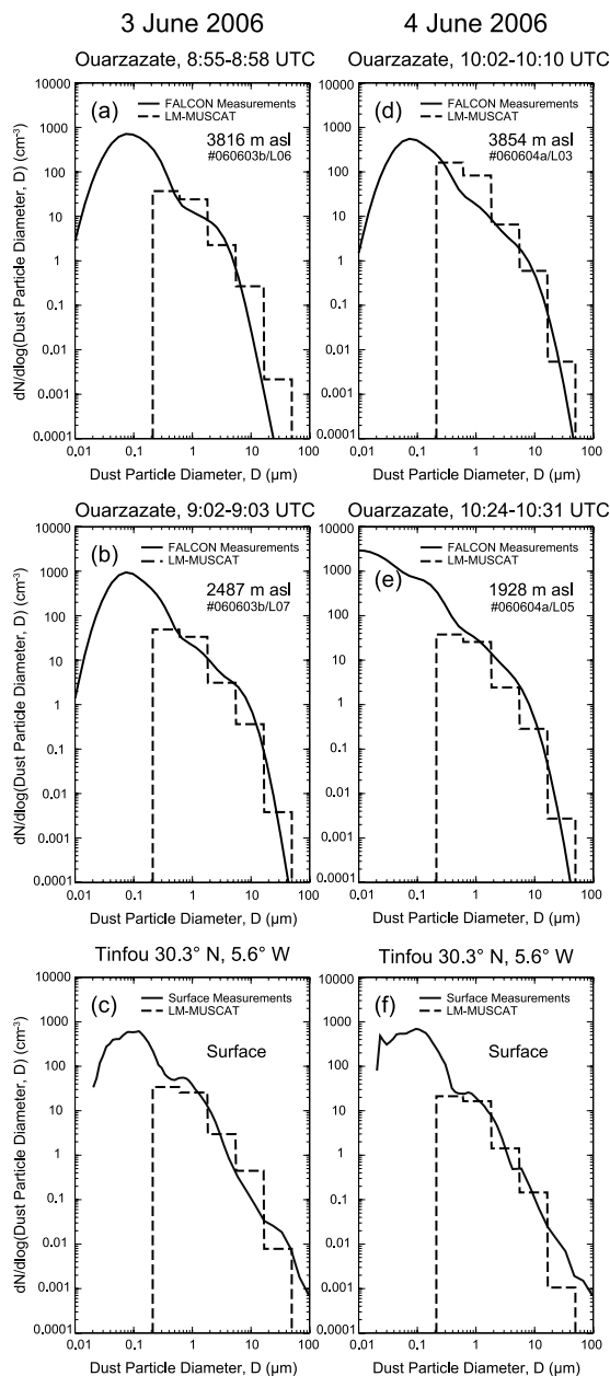
Fig. 9. Comparison of the number size distribution above Ouarzatete at different heights on 3 June 2006 (around 9:00 UTU; a, b) and 4 June 2006 (around 10:00 UTC; d, e). Particle size distribution from airborne measurements aboard Falcon aircraft (solid line) and model results (dashed line). Ground-level number size distribution at the SAMUM site Tinfou on 3 June (11:13 UTC) and 4 June 2006 (9:50 UTC). Model results of the first layer at about 35 m height (dashed line), measurements from a combined DMPS/APS system at about 5 m height (solid line) (c, f).
