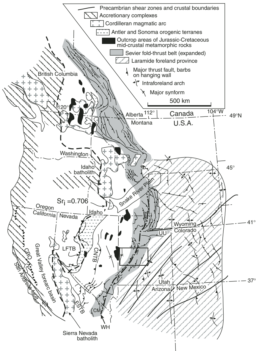
Figure 1. Generalized tectonic map of the western United States showing the major elements of the Cordilleran orogenic belt (modified after DeCelles, 2004). The initial Sr_i ratio line ( Sr_i ) is from Armstrong et al. (1977) and Kistler and Peterman (1978). Abbreviations are as follows: LFTB—Luning-Fencemaker thrust belt; CNTB—Central Nevada thrust belt; ESTB—East Sierran thrust belt; UU—Uinta Mountains uplift; WH—Wasatch hinge line; CM—Clark Mountains; CRO—Coast Range Ophiolite. Study area is outlined by rectangle in central Utah. Precambrian shear zones are after Karlstrom and Williams (1998).
