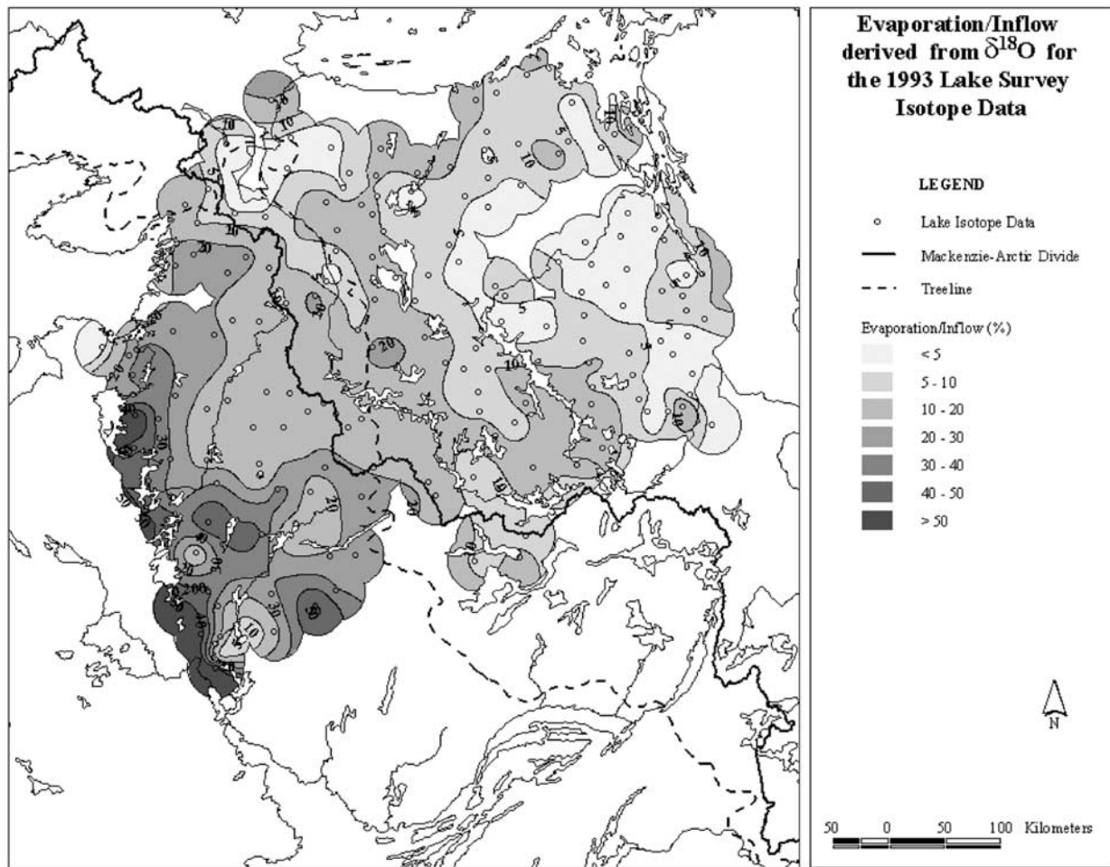
Figure 8. Map showing E/I ratios (%) for lakes based on 1993 sampling. See color version of this figure at back of this issue.
