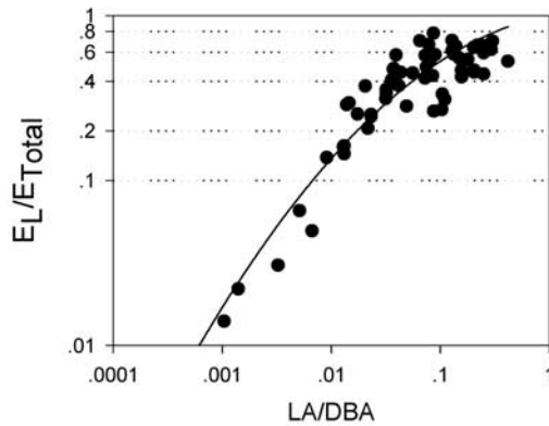
Figure 9. Relationship between lake area/drainage area ratios and E_L/E_{\text{Total}} (or fraction of water loss from sampled lake versus all lakes in catchment area) for a subset of 60 lakes. Note that LA refers to area of sampled lake only (not including upstream lakes) and all lakes can be classified as nonheadwater lakes (that is, contributing area contains appreciable open water). Note that lakes in large basins have minor influence on evaporation loss signal. Where lake area exceeds 10% of basin area, lake evaporation becomes dominant signal.
