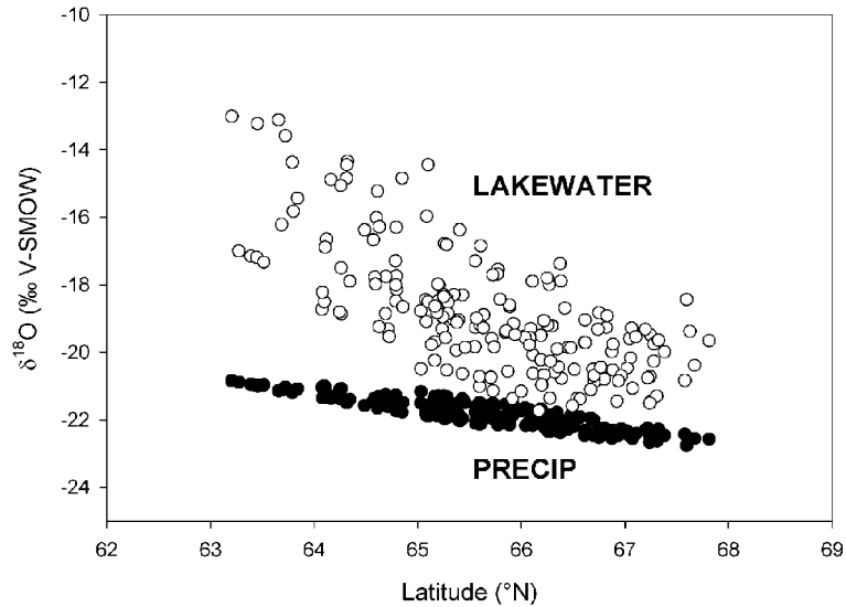
Figure 6. Plot of latitudinal variations of lake water (open circles) sampled during 1993 (from Figure 2) and GNIIP mean annual precipitation (solid circles) for each lake site (interpolated from Figure 5a). Note that latitudinal trends in isotopic composition of lake water are larger than variations in precipitation, which is attributed to higher evaporation losses at lower latitudes.
