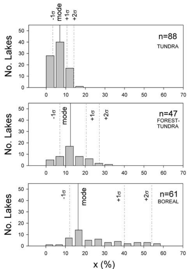
Figure 12. Frequency of lakes with specified fraction of water loss by evaporation, shown separately for each major terrain unit. Note systematic decrease in mode of x from boreal to tundra environments. Distributions are all right-skewed, and variability in evaporation loss ( x ) decreases progressively from boreal forest to tundra.
