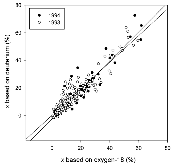
Figure 7. Evaporation/inflow x based on deuterium (%) versus x based on oxygen-18 (%) for lakes sampled in 1993 and 1994. Good agreement between oxygen-18 and deuterium suggests that basic model exchange parameters are adequately defined. Note that 1994 survey area included several lakes near Great Slave Lake that were not sampled in 1993. These lakes have the highest x values observed.
