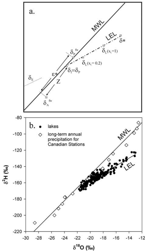
Figure 1. Plots of ^2H - ^{18}O (a) showing schematic relationships between isotopic compositions in surface water systems including limiting isotopic enrichment ( \delta^* ), mean annual input ( \delta_I = \delta_P ), lake water \delta_L under two water balance scenarios where x = 1 and x = 0.2 , and atmospheric moisture ( \delta_A^{fw} ) estimated assuming equilibrium with flux-weighted precipitation ( \delta_P^{fw} ) and noting that Z = \delta_I - \delta_A^{fw} , which is apparent inflow-atmospheric moisture separation, and (b) showing lakes sampled in central Arctic and precipitation from Canadian stations. Note that lakes plot along an evaporation line (LEL) with a slope of 4.7 ( r^2 = 0.88 ) and precipitation plots close to meteoric water line (MWL) of \delta^2H = 8\delta^{18}O + 10 . Isotopic composition of lakes is controlled predominantly by variations in evaporation loss from lake and upstream lakes.
