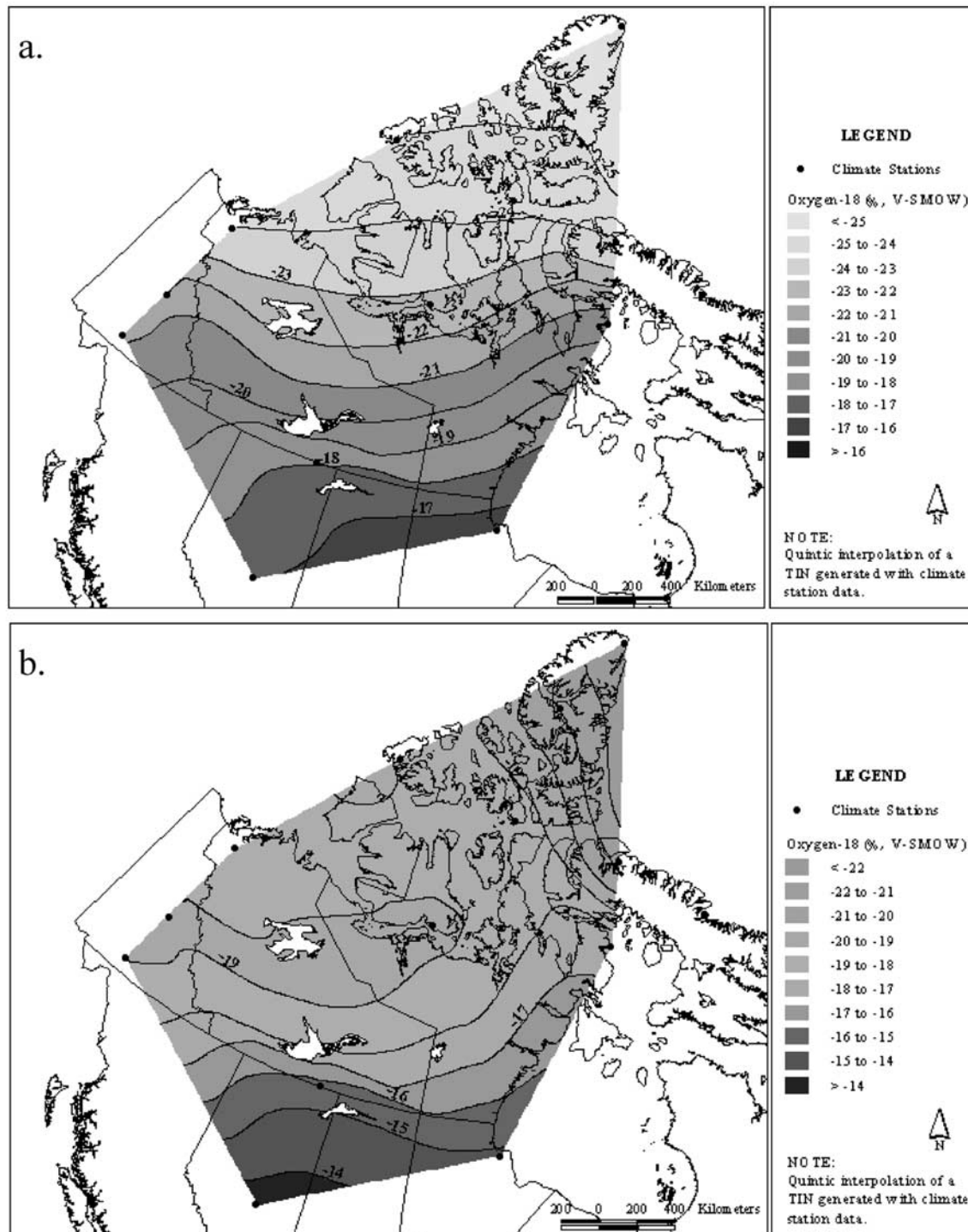
Figure 5. Map showing \delta^{18}\text{O} composition of (a) mean annual precipitation and (b) evaporation-flux-weighted (thaw season) precipitation, interpolated from nearby Global Network for Isotopes in Precipitation (GNIP) stations. Similar trends are noted for \delta^2\text{H} . See color version of this figure at back of this issue.
