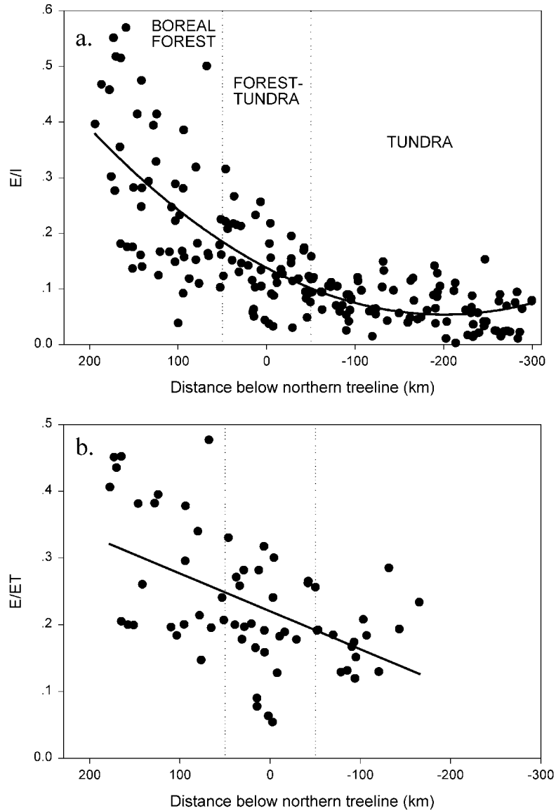
Figure 10. Southwest-northeast (boreal-tundra) variations in water balance ratios estimated by oxygen-18 mass balance. (a) Fraction of water loss by evaporation. (b) Fraction of total evapotranspiration loss by evaporation. Boreal forest, forest-tundra transition, and tundra regions are defined approximately based on distance below northern tree line.
