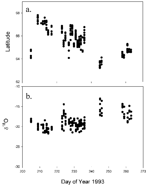
Figure 3. 1993 time series of (a) water sampling latitude and (b) \delta^{18}\text{O} , showing that temporal changes in isotopic composition are related to latitude rather than due to substantial seasonal differences in isotopic enrichment.
