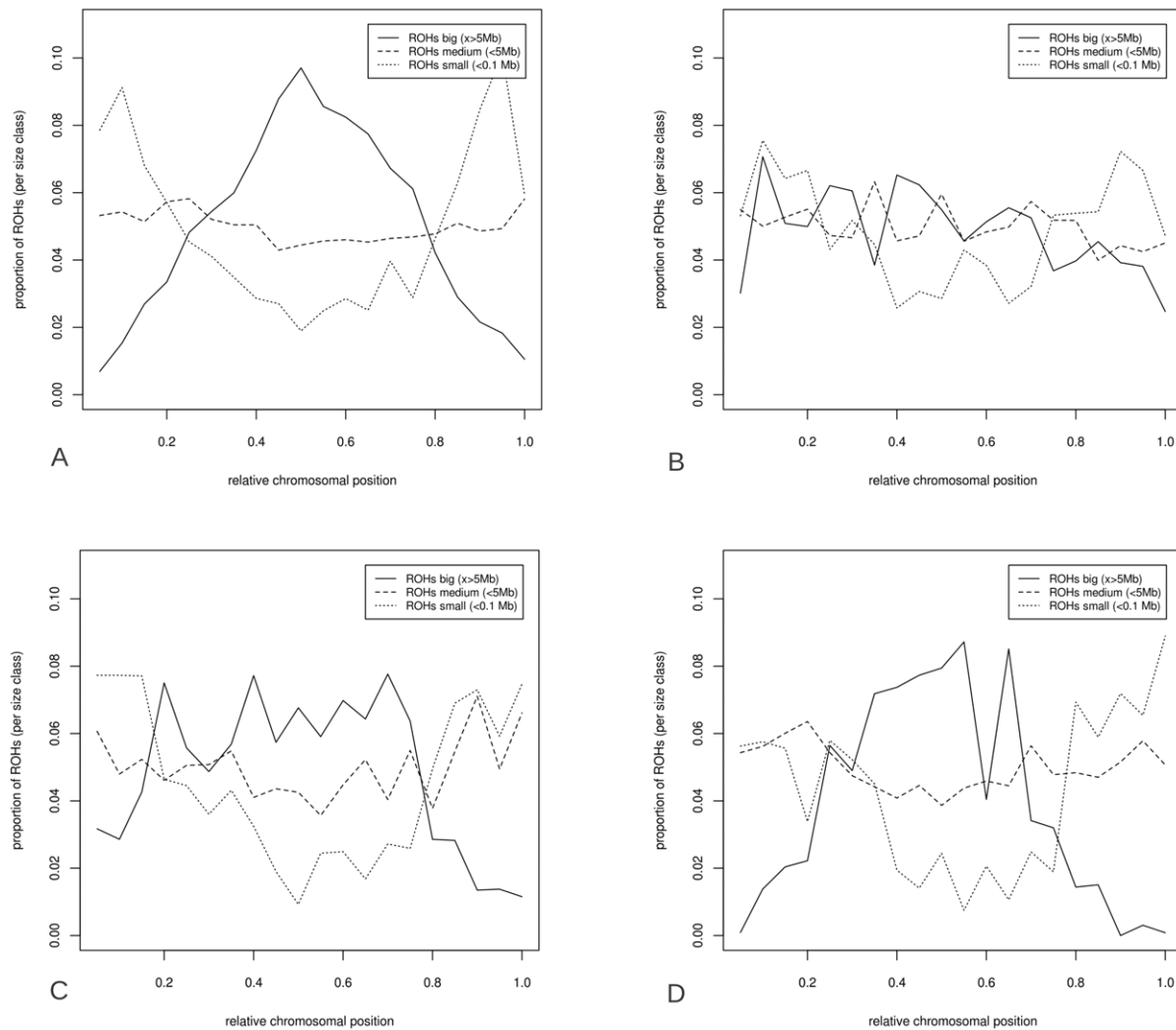
Figure 7. Distribution of ROHs over relative chromosomal position. ROHs were split into three size classes; big ( >5 Mbp), medium (0.1 to 5 Mbp) and small ( <0.1 Mbp). The distribution is relative only to the total number of ROH bins in that particular size class, and the distributions are averaged over all chromosomes. ROH distribution is given for four groups: European pigs (7A), European wild boars (7B), Asian pigs (7C) and Asian wild boars (including the Japanese, 7D). doi:10.1371/journal.pgen.1003100.g007
