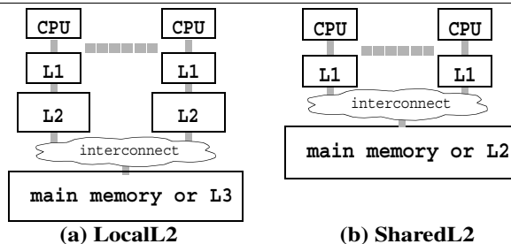
Figure 1: Two shared memory multiprocessor models. (a) LocalL2 : local L1 and L2 caches and a shared L3. (b) SharedL2 : local L1 caches and a shared L2. The interconnect is functionally a bus but may be implemented via other components [11].
