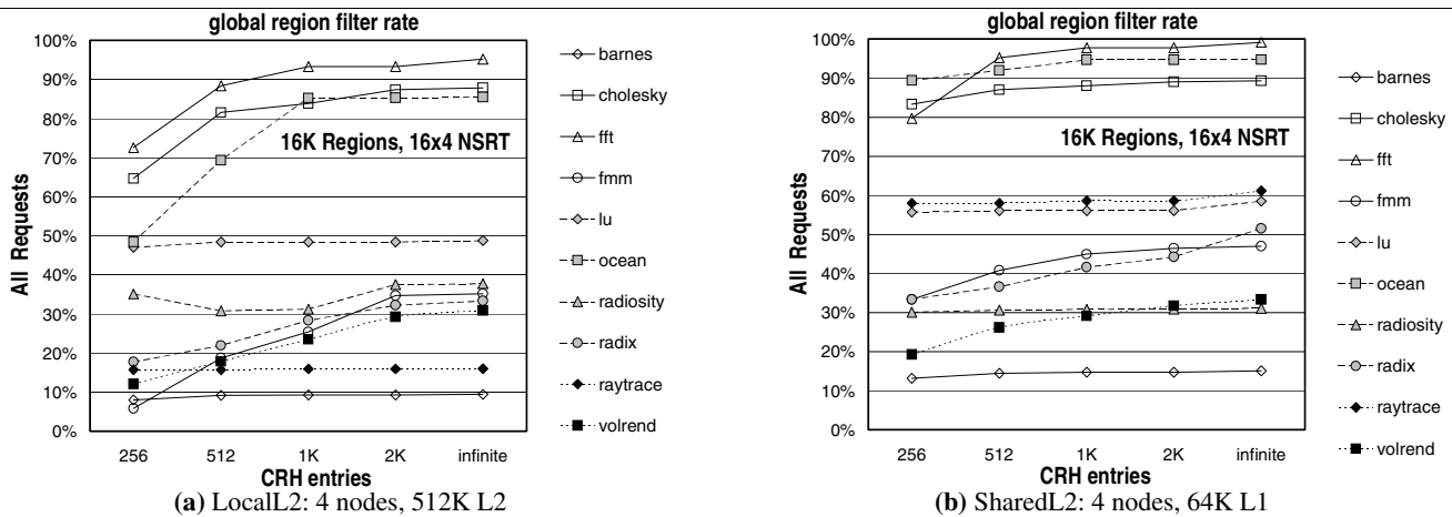
Figure 7: Filter rates per program for 16K byte regions on four node systems with 512K L2 (a) and 64K L1 (b) caches respectively. The NSRT is fixed at 64 entries (16 sets, 4-way set-associative) and the number of CRH entries varies as shown on the X-axis.
