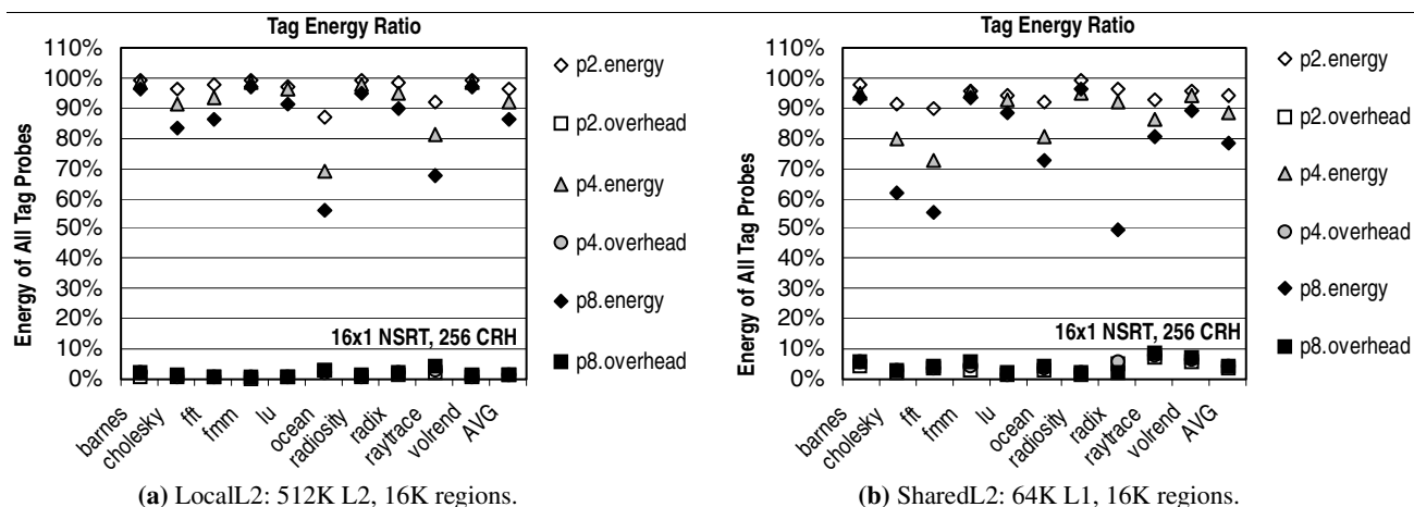
Figure 11: Tag energy ratio and RegionScout energy overhead. 16K Region, 16-entry direct-mapped NSRTs and 256-entry CRHs.
