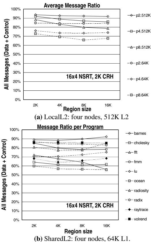
Figure 9: Avoiding broadcasts with RegionScout for various region sizes. NSRT is 64-entries, 4-way set-associative and the CRH has 2K entries. Shown is the ratio of messages sent with RegionScout over those sent without it. (a) Average message ratio for LocalL2 and SharedL2 systems with 512K L2 and 64K L1 caches respectively. (b) Message ratio per program for the SharedL2 system with 64K L1 caches.
