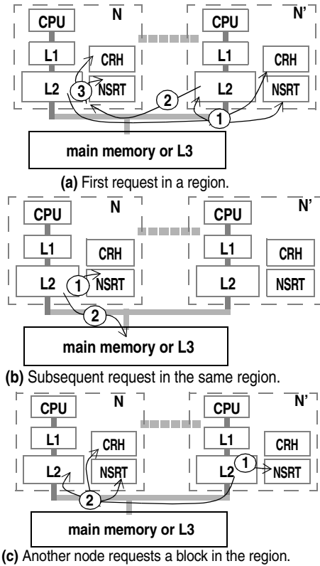
Figure 3: An example illustrating how RegionScout works. Without the loss of generality we use the LocalL2 model and show only two nodes. (a.1) Node N requests block B in region RB. The request is broadcast to all nodes (N first checked its NSRT and since it was empty it found no matching entry for region RB). (a.2) All remote nodes probe their CRH and report that they do not cache any block in region B. (a.3) Node N records RB as not shared and increments the corresponding CRH entry. (b.1) Node N is about to request block B' in region RB and first checks that its NSRT. (b.2) Since an entry is found the request is sent only to main memory. (c.1) Node N' requests block B'' in region RB. It first checks its NSRT. (c.2) Since the region is not recorded in its NSRT, it broadcasts its request. Node N invalidates its NSRT entry since now RB is shared.
