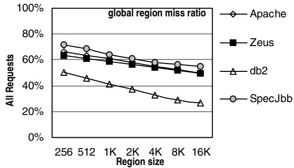
Figure 12: (a) Global Region Miss ratios for four commercial application workloads with the LocalL2 model and 512K L2 caches and 16 processors.
