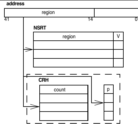
Figure 4: NSRT and CRH organization for 16Kbyte regions.
