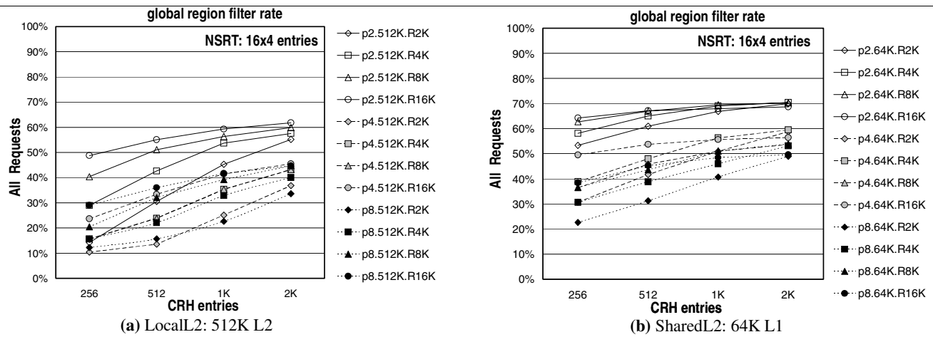
Figure 6: Average global region miss filter rates (see text for the definition) for various CRH sizes (X-axis). The NSRT has 64 entries organized in 16 sets of four entries each. The curves correspond to systems with different number of nodes N and to different region sizes S as identified by the pN.C.RS labels. C is the size of the L2 and L1 caches for models LocalL2 (a) and SharedL2 (b) respectively.
