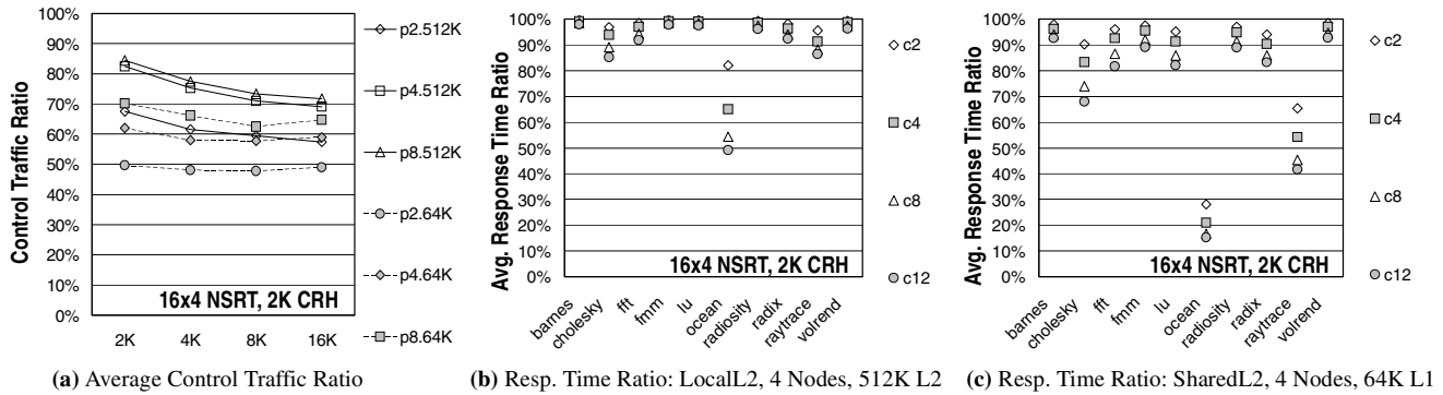
Figure 8: (a) Relative control traffic for the bus-based interconnect model. Reported is the ratio of the average control traffic for the system with RegionScout over the base system. (b) and (c): Estimated average snoop response time ratio with RegionScout over the base system for LocalL2 and SharedL2 respectively. We report results for various snoop processing latencies. Per snoop latency is modelled in N processor cycles (labels cN ) where N is 2, 4, 8 or 12. The NSRT has 64-entries and is 4-way set-associative and the CRH has 2K entries.
