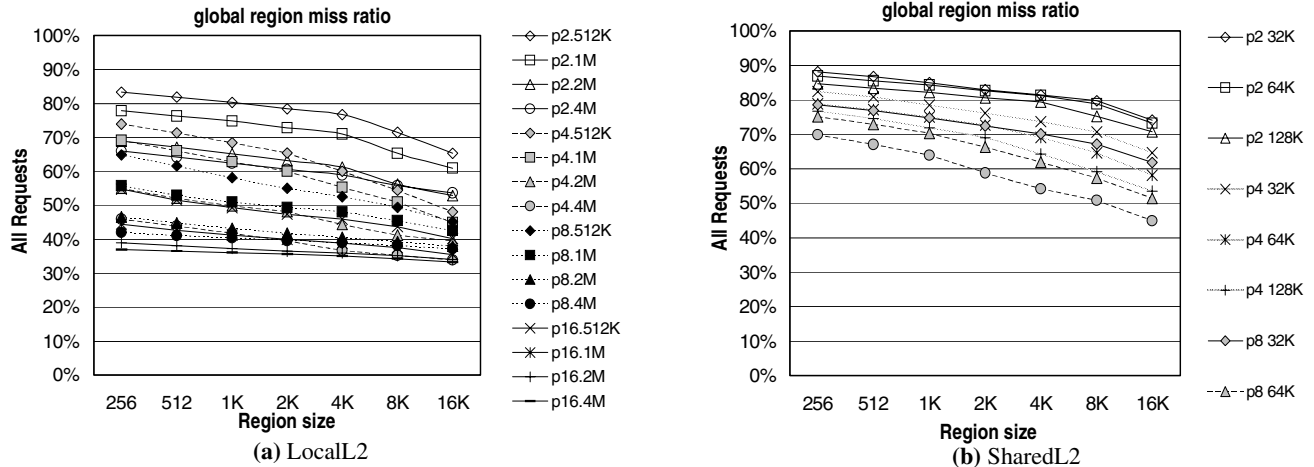
Figure 2: Average global region miss ratio for various shared memory multiprocessor systems (different curves) and region sizes (X-axis). (a) Systems with local L1 and L2 caches and shared L3. (b) Systems with local L1 caches and a shared L2. Labels are pN.S where N is the number of nodes and S is the L2 and L1 cache size for parts (a) and (b) respectively.
