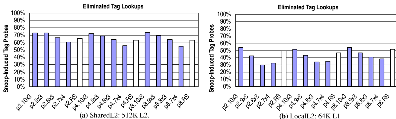
Figure 10: Snoop-induced tag lookups avoided with Jetty and RegionScout. The RegionScout filter used comprises a 256-entry CRH and a 16-entry 2-way set-associative NSRT and uses 16K regions. See text for a description of the four hybrid Jetty filters. We use a pN.filter naming scheme where N is the number of nodes and filter can be a Jetty (10x3, 9x3, 8x3 or 7x4) or RegionScout (RS).
