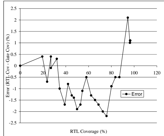
Figure 4 Module M3: Error v/s Fault Coverage
