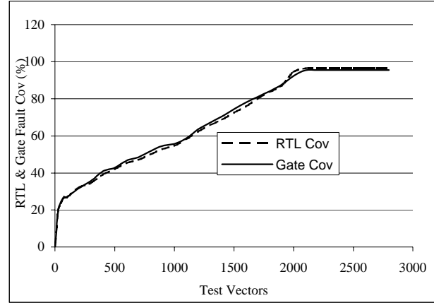
Figure 3 Module M3: RTL and Gate Cov. v/s Test Vectors
