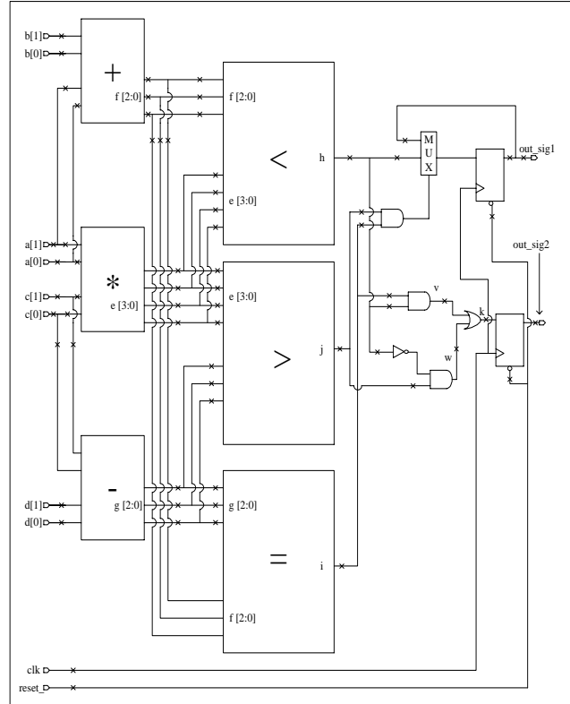
Figure 1 RTL Faults in a Schematic Representation
