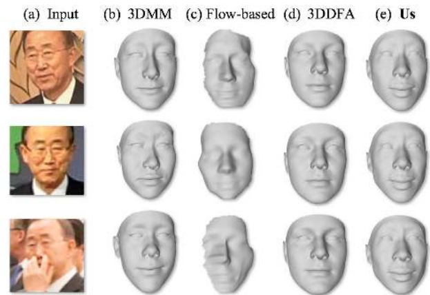
Figure 1: Unconstrained, single view, 3D face shape reconstruction. (a) Input images of the same subject with disruptive poses and occlusions. (b-e) 3D reconstructions using (b) single-view 3DMM [33], (c) flow based method [13] (d) 3DDFA [47], (e) Our proposed approach. (b-c) Present different 3D shapes for the same subject and (d) appears generic, whereas our method (e) is robust, producing similar discriminative 3D shapes for different views.
