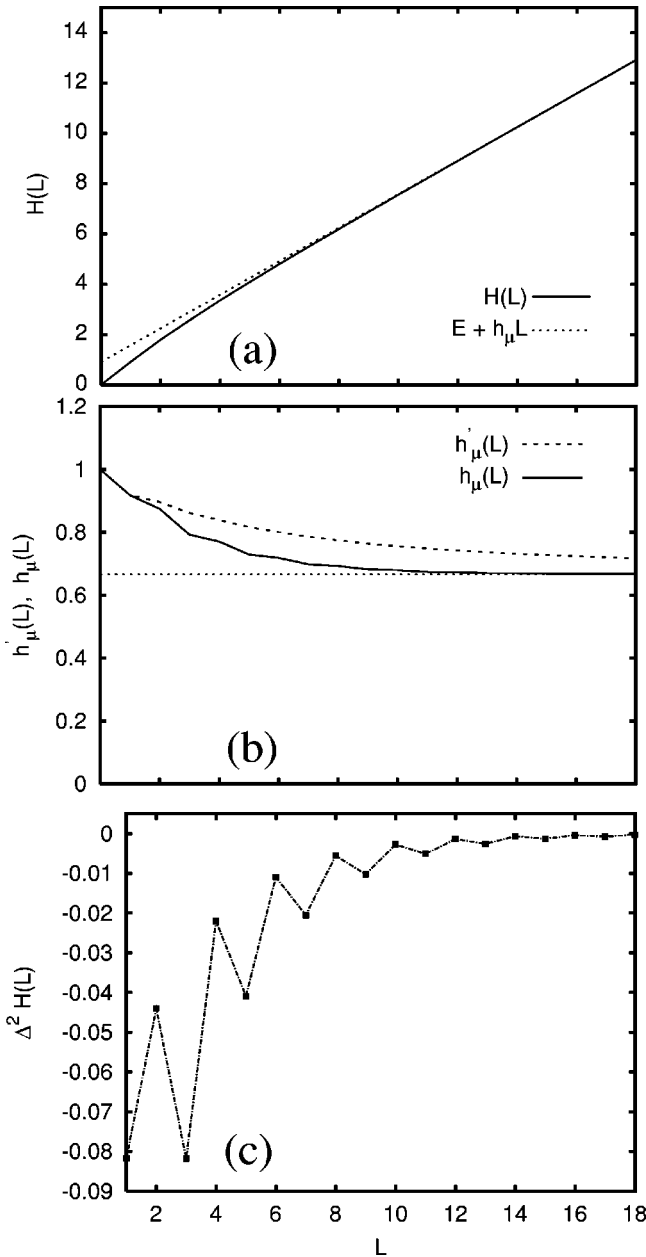
FIG. 11. (a) Entropy growth (solid line) for the even process, along with the asymptote E + h_\mu L (dotted line). (b) Entropy convergence, both h_\mu(L) (solid line) and h'_\mu(L) (dashed line), and h_\mu (dotted line) for the same. (c) Predictability gain \Delta^2 H(L) vs sequence length.
