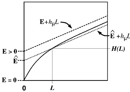
FIG. 20. Assumed synchronization leads to less apparent memory: Schematic illustration of how assuming synchronization to a source, in this case implicitly assuming H(L) = E + h_\mu L , leads to an underestimate \hat{E} of the actual memory E > 0 .
