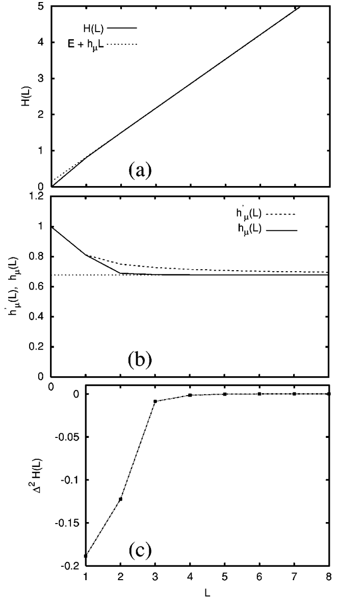
FIG. 13. (a) Entropy growth (solid line) for the simple nondeterministic source, along with the asymptote E + h_\mu L (dotted line). (b) Entropy convergence, both h_\mu(L) (solid line) and h'_\mu(L) (dashed line), and h_\mu (dotted line) for the same. (c) Predictability gain \Delta^2 H(L) vs sequence length.
