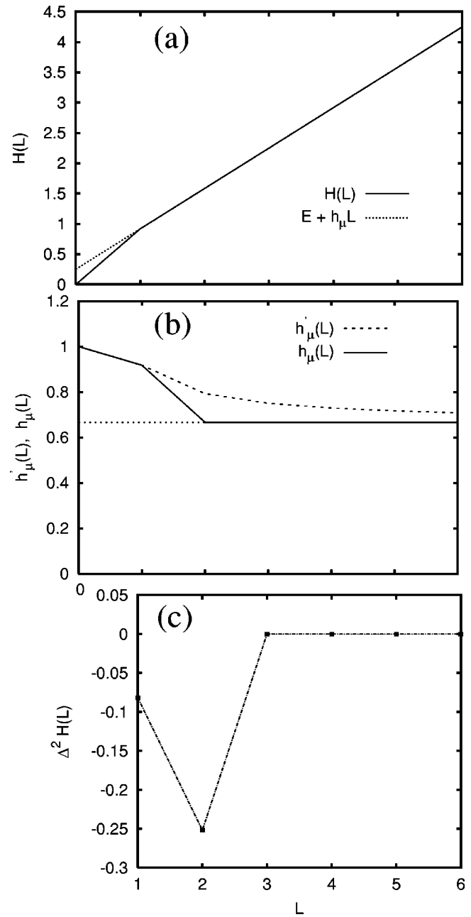
FIG. 8. (a) Entropy growth (solid line) for the golden mean process, along with the asymptote \mathbf{E} + h_\mu L (dotted line). (b) Entropy convergence, both h_\mu(L) (solid line) and h'_\mu(L) (dashed line), and h_\mu (dotted line) for the same. (c) Predictability gain \Delta^2 H(L) vs sequence length.
