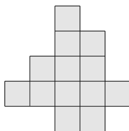
(A) L -convex polyomino \mathcal{P}
