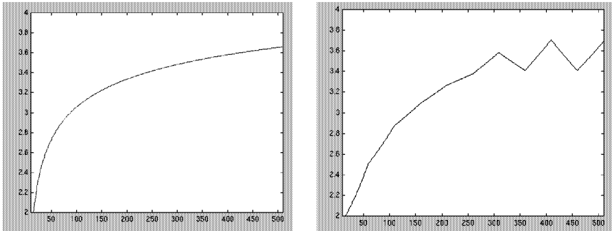
Figure 1. An experiment (suggested by V. Vapnik) where the optimal \lambda does not simply depend on the training set as \lambda = \alpha/l with \alpha a constant and l the number of data points in the training set. In the right figure we plot \lambda l as a function of the number of data. The data were generated from a 1-D sinusoid along 3 periods, with small uniform noise added. A SVMR with Gaussian kernel was used. We scaled the ordinate by 50 to compare with the \log(\log(l)) plot shown on the left. The number of training data ranged from 10 to 500. For each l we plot \lambda l with \lambda being the optimal one (i.e., 2/C for the SVMR) estimated by using the true function for validation. The right figure shows that \lambda l is not a constant as the MAP interpretation would require.
