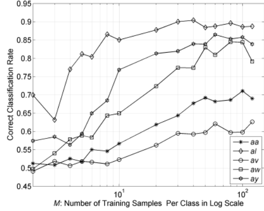
(a) The CCRs obtained by CSP for each of the five subjects.
