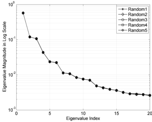
(b) The eigenvalue distribution of a typical average covariance matrix with regularization \beta = 0.3 .
