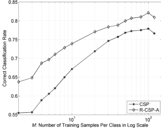
Fig. 5. Illustration of the improvement achieved over CSP by the proposed R-CSP-A algorithm in Experiment I.
