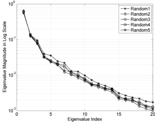
(a) The eigenvalue distribution of a typical average covariance matrix without regularization by \beta .
