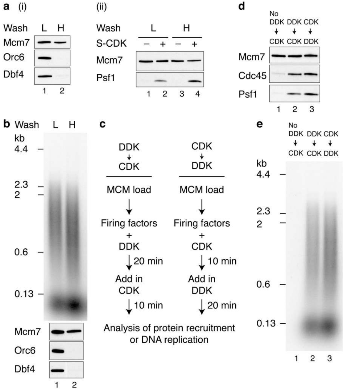
Figure 6. DDK phosphorylation of MCM promotes origin firing either before or after S-CDK. a. Reactions performed essentially as in Fig. 1b on circular DNA but with an additional mid-reaction wash immediately following DDK phosphorylation, in either a low salt (L) (0.3 M K-glu), or high salt (H) (0.6 M NaCl) buffer. Bound proteins immediately following the mid-reaction wash (i), and after firing factor recruitment followed by 0.3 M KCl washes (ii). b. Replication reactions with either high or low salt mid-reaction washes. c. Reaction schemes to test the order of DDK and CDK action. Firing factor recruitment was performed in a
