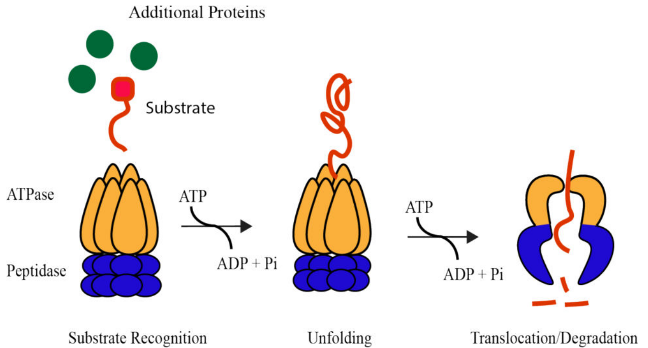
Figure 1. Energy-dependent proteases are composed of an ATP-hydrolysis active unfoldase domain and a chambered peptidase domain. Through successive rounds of ATP hydrolysis, a specific substrate protein is selected by the protease, unfolded by the ATPase domain, and translocated through a central pore to the peptidase chamber where it is degraded.
