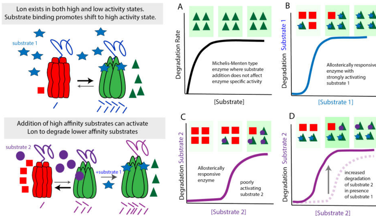
Figure 3. Lon is subject to allosteric regulation (a) Many proteases, such as ClpXP and ClpAP, adhere to typical Michaelis-Menten kinetics where adding increasing amounts of substrate leads to an increase in the rates of degradation until the protease becomes saturated and V_{max} is reached resulting in the classic hyperbolic curve. (b) This contrasts with Lon which exhibits positive cooperativity upon increasing substrate concentration. The working model is that Lon exists as low (red triangles) and high activity (green squares) states with substrate binding promoting the highly active state. (b) In the case of substrate 1, which has a strong affinity for Lon, relatively low amounts of substrate are needed to shift Lon to the active state. (c) Substrate 2 binds Lon poorly and activation requires much higher concentrations of substrate 2. (d) If the concentration of substrate 2 is kept the same and the high affinity substrate 1 is added, Lon will be shifted to the active form, leading to robust degradation of the normally poorly degraded substrate 2.
