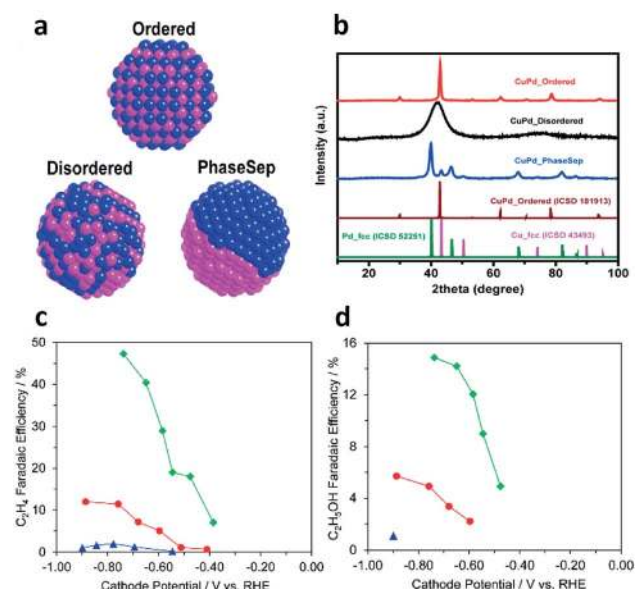
Fig. 12 (a) Schematic illustration of CuPd nanoalloys with ordered, disordered and phase-separated structures. (b) XRD patterns of the prepared CuPd nanoalloys. Faradaic efficiencies of (c) C 2 H 4 and (d) C 2 H 5 OH for bimetallic Cu–Pd catalysts with different mixing patterns: ordered, blue; disordered, red; phase-separated, green. Reprinted from ref. 87 with permission from American Chemical Society.
