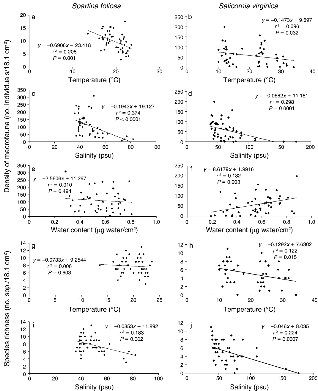
FIG. 4. Regressions showing relationships between macrofauna density and (a, b) temperature, (c, d) salinity, and (e, f) water content; and between macrofaunal species richness and (g, h) temperature and (i, j) salinity. Data were pooled across treatments and seasons.
