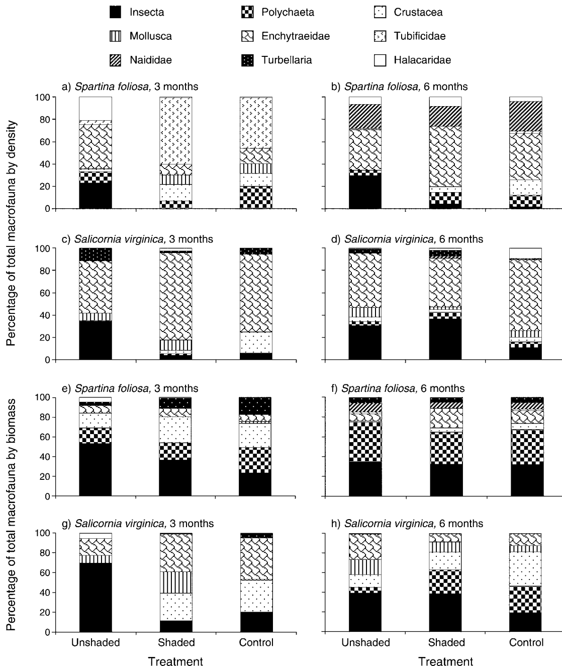
FIG. 3. Macrofaunal community composition (a–d) based on counts or (e–h) based on biomass in three treatments three and six months after experiment initiation: unshaded (absence of plant cover and structure), shaded (absence of plant structure), and control (plants intact) in Spartina foliosa and Salicornia virginica treatment plots.
