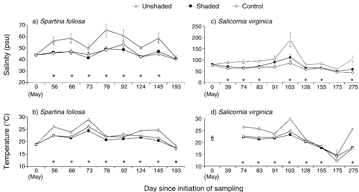
FIG. 1. Porewater salinity (practical salinity units, psu) and temperature (mean \pm SE) of upper 2 cm of sediment in three treatments in Spartina foliosa and Salicornia virginica treatment plots. Values designated with asterisks indicate that unshaded treatment values are significantly different from shaded and control treatment values (Wilcoxon rank sum, P < 0.05 ). The research was conducted in the 6.5-ha Kendall Frost Mission Bay Marsh Reserve, an intertidal salt marsh in the northeast corner of Mission Bay, San Diego, California, USA. Temperature data were not collected on day 39 in S. virginica habitat due to equipment malfunction.
