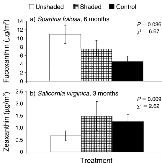
FIG. 2. Pigment abundance (mean \pm SE) of (a) fucoxanthin in Spartina foliosa at six months and (b) zeaxanthin in Salicornia virginica at three months as determined through high-performance pigment chromatography: only significant ( P < 0.05 ) results are shown. Letters indicate a posteriori differences among treatments ( P < 0.05 ) in pigment abundance values. Graphs indicate increased importance of diatoms in unshaded treatment plots relative to control and shaded treatment plots.
