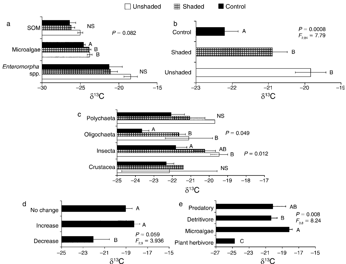
FIG. 5. Stable isotope signatures ( \delta^{13}\text{C} ; mean \pm SE) of sediment, microalgae, macroalgae, and selected macrofauna in Salicornia virginica habitat 11 months after treatment initiation. Natural abundance \delta^{13}\text{C} values are given for (a) macrofaunal food sources (SOM, sediment organic matter), (b) total combined macrofauna, (c) major macrofaunal taxa, (d) macrofauna grouped by response to unshaded treatment, and (e) macrofauna grouped by feeding mode. Uppercase letters to the right of error bars indicate significant ( P < 0.05 ) a posteriori differences in \delta^{13}\text{C} values among treatments.
