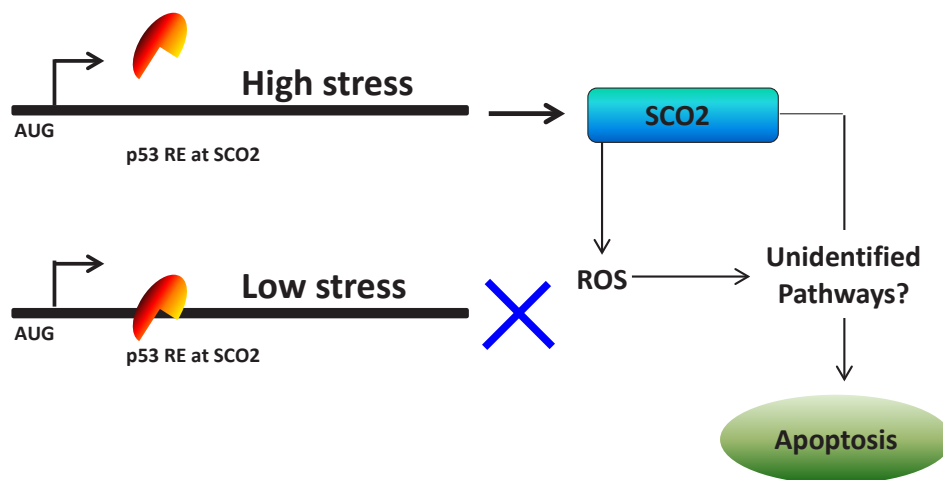
Figure 1b: A model depicting the mechanism of p53-mediated regulation of SCO2 gene in cancer cells.
