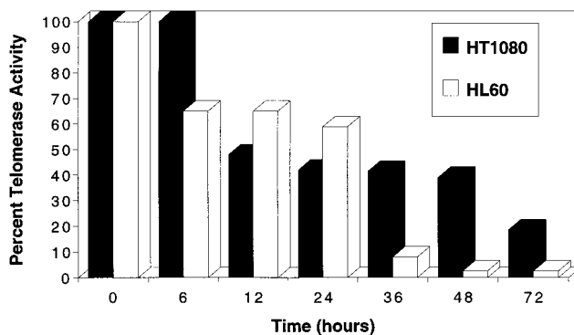
FIG. 2. Half-life of telomerase activity in cycloheximide-treated cells. HT1080 and HL60 cells were treated with a final concentration of 300 \mu g of cycloheximide per ml for 72 h. Cells were harvested at the indicated times and tested for telomerase activity by the TRAP assay. Quantitation of telomerase activity in the cycloheximide-treated cells was done by determining the ratio of ITAS to telomerase activity. The subsequent levels of telomerase activity are represented as a fraction of the 0-h activity.
