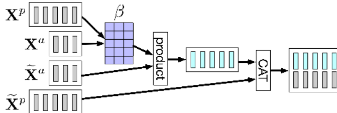
Figure 2: The attention-based soft-alignment mechanism.
