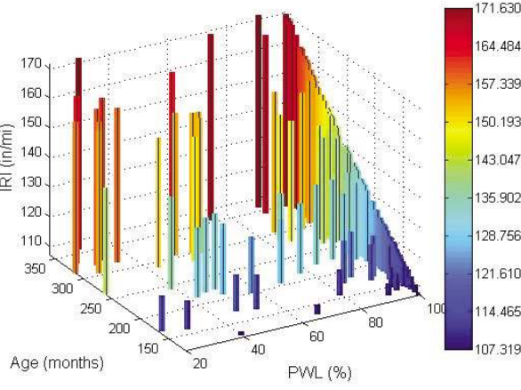
Fig. 3. Pavement performance versus PWL (in-situ air voids) for mix 1 using MEPDG results
