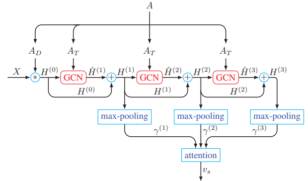
Figure 3: Overview of LST-AGCN.
