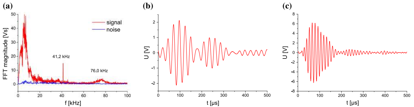
Fig. 11 a Frequency spectrum of the exemplary electromagnetic signal and, for comparison, an exemplary noise measurement ( blue ). b and c Temporal characteristics of the components labelled in the spectrum. b Signal with 40–42 kHz bandpass filter. c Signal with 65–85 kHz bandpass filter
