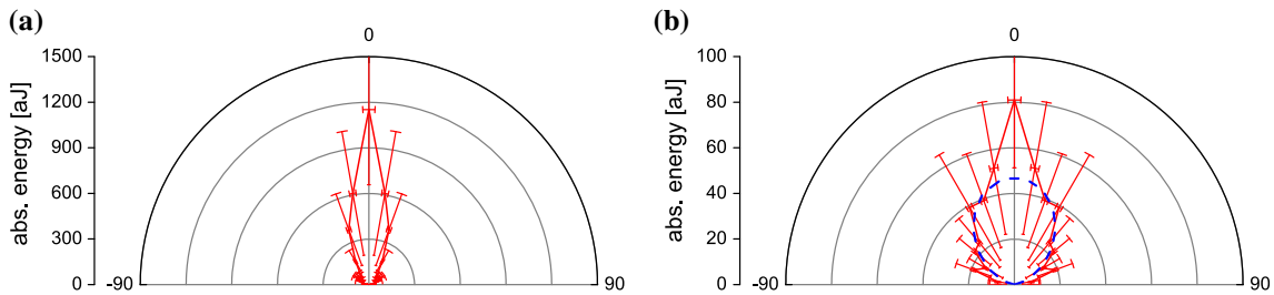
Fig. 12 Signal properties depending on detection angle. The data is mirrored at the 0° axis for clearness. a Angular dependence of the absolute energy of the whole signal. b Angular dependence of the absolute energy of the oscillating part of the signals and a scaled \cos^2(\phi) graph ( dashed )
