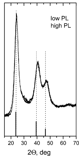
Figure 4. Powder X-ray diffractograms of highly and lowly luminescent CdTe nanocrystals of the same size. The line spectrum corresponds to the cubic phase of bulk CdTe.
