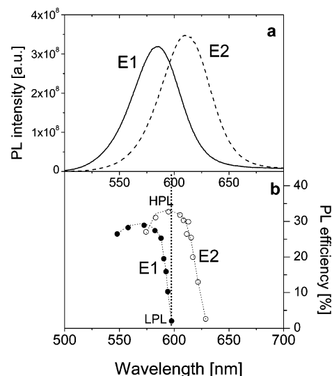
Figure 2. Photoluminescence spectra of the crude solution of CdTe nanocrystals (a). Spectra of the same ensemble are shown after two different times of refluxing where the dashed curve “E2” corresponds to a longer refluxing time. Part (b) shows the quantum efficiency of monodispersed fractions of portions of the ensembles “E1” and “E2”. The lowly luminescent fraction “LPL” of the ensemble “E1” has the same particle size as the highly luminescent fraction “HPL” of the ensemble “E2”.
