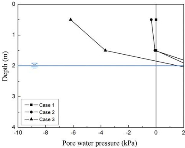
Fig. 9. Pore water pressure of depth 4.0 m.
