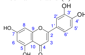
Luteolin (4)
