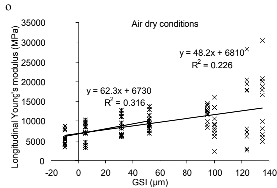
Fig. 8. Relation between Longitudinal Young's modulus and GSI. wet conditions and air dry conditions. × : all GSI ; * : GSI < 60µm.
