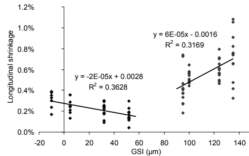
Fig. 6. Disjunct relation between longitudinal shrinkage and GSI.
