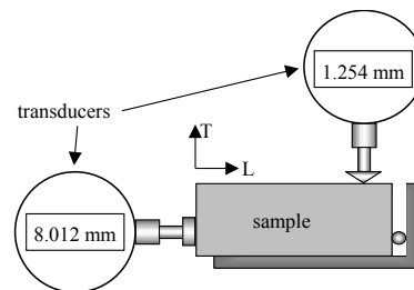
Fig. 3. Apparatus for measuring dimension changes of samples.
