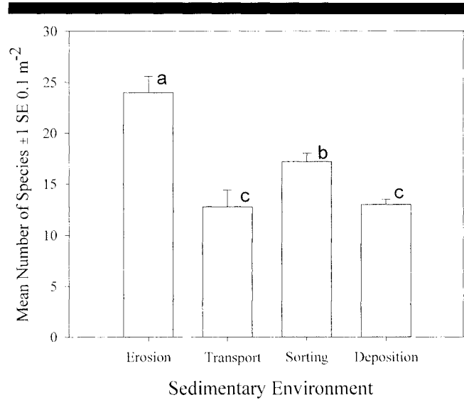
Figure 5. Mean number of species 0.1 m 2 in different sedimentary environments estimated from PELLEGRINO and HUBBARD'S (1983) survey data. Station data were sorted by sedimentary type using a geographic information system and then analyzed using one-way analysis of variance and a post-hoc Bonferroni multiple comparison test (HINTZE, 1997). Differences among sedimentary environments were highly significant ( F_{3,395} = 23.81 , MSE = 1.181 , p < 0.0001 ). Lowercase letters on data bars indicate results of post-hoc tests with matching letters indicating no significant differences ( p > 0.05 ) in species richness.
