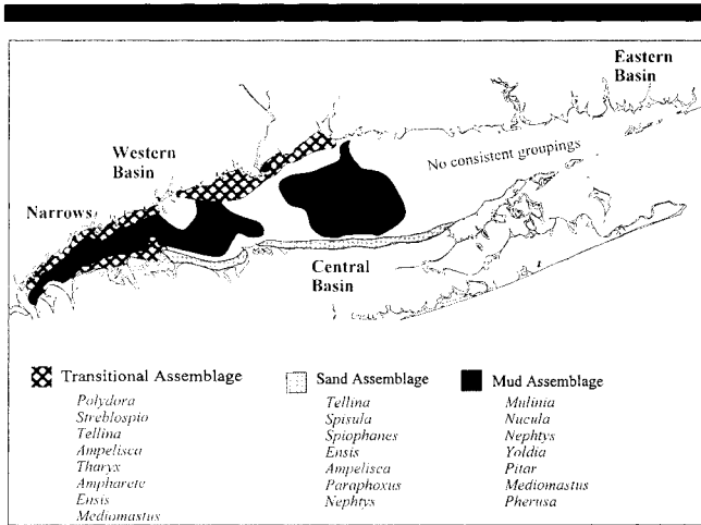
Figure 4. Infaunal community types recognized by REID et al. (1979) in Long Island Sound. Dominant species are given below each assemblage type in decreasing order of average abundance. Each group of species comprised 60 to 90% of the total abundance within the designated assemblage.
