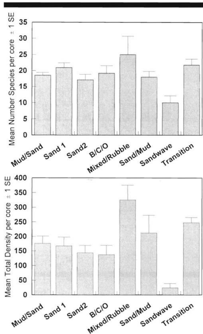
Figure 13. Mean ( \pm 1 standard error) total species per core and total abundance in each of the large-scale sea-floor elements in the sidescan mosaic study area. Differences among elements were significant for both total abundance ( F_{7,49} = 4.23 , MSE = 7554.2 , P < 0.001 ) and species richness ( F_{7,49} = 3.56 , MSE = 24.6 , p < 0.01 ).
