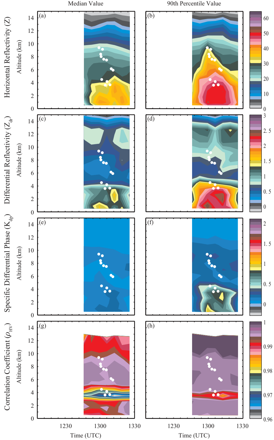
FIG. 2. Median (left column) and 90th percentile (right column) radar values for each radar elevation angle within a 10 km square box centered on the small, short-lived cell. The 90th percentile is calculated by determining the radar value at which 90% of the data occurs below that value for each radar elevation angle. The locations at which lightning was initiated within the cell are indicated by white circles. (a-b) horizontal reflectivity Z , (c-d) differential reflectivity Z_{dr} , (e-f) specific differential phase K_{dp} and (g-h) correlation coefficient \rho_{HV} .
