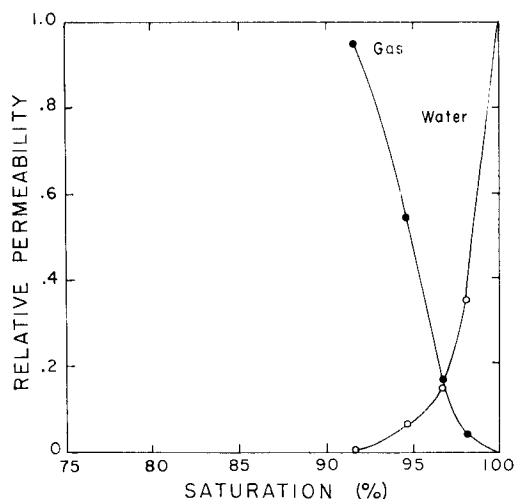
FIG. 3. Typical relative permeability curve of a ring-porous specimen (American elm) obtained from drainage-type measurements.
