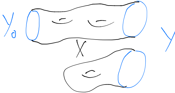
FIGURE 1. A geometric bordism X: Y_0 \rightarrow Y_1
