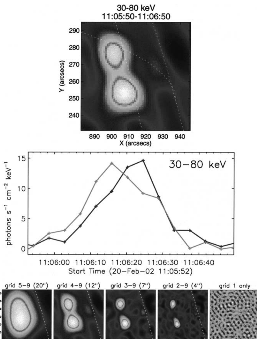
Figure 2. Non-thermal X-ray image (30–80 keV) of the 20 February flare with a resolution of 12'' ( top ). At this resolution, only two sources are seen that show different time profiles (in gray for the northern source) suggesting non-simultaneous brightening of footpoints ( middle ). Cleaned images with successively better resolution are shown below. The last image is computed using the finest grid only (grid 1, 2.3'' ) and does not show significant emission. All times in UT.
