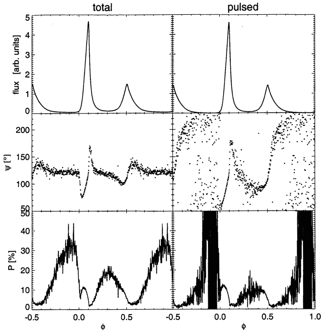
Fig. 6.— Preliminary optical data on the Crab pulsar obtained with the OPTIMA instrument (Kanbach et al. 2003). Left column: a lightcurve (top panel), a position angle \psi (dots, middle panel), and a degree of polarization P (bottom panel). The constant value of position angle within phase ranges 0.6 – 0.9 and 1.1 – 1.2 suggests that the received radiation consists of two components, one of which has constant properties. Right column: same as in the left column but with the contribution of the constant component subtracted from the data. Following Kellner (2002), for the constant component we assumed intensity equal to 1.24 % of the maximum intensity of the total signal, \psi = 123^\circ , and P = 33\% . One and a half period is shown. The maximum of the leading peak was aligned with the phase \phi = 0.1 . The data were kindly provided by G. Kanbach.
