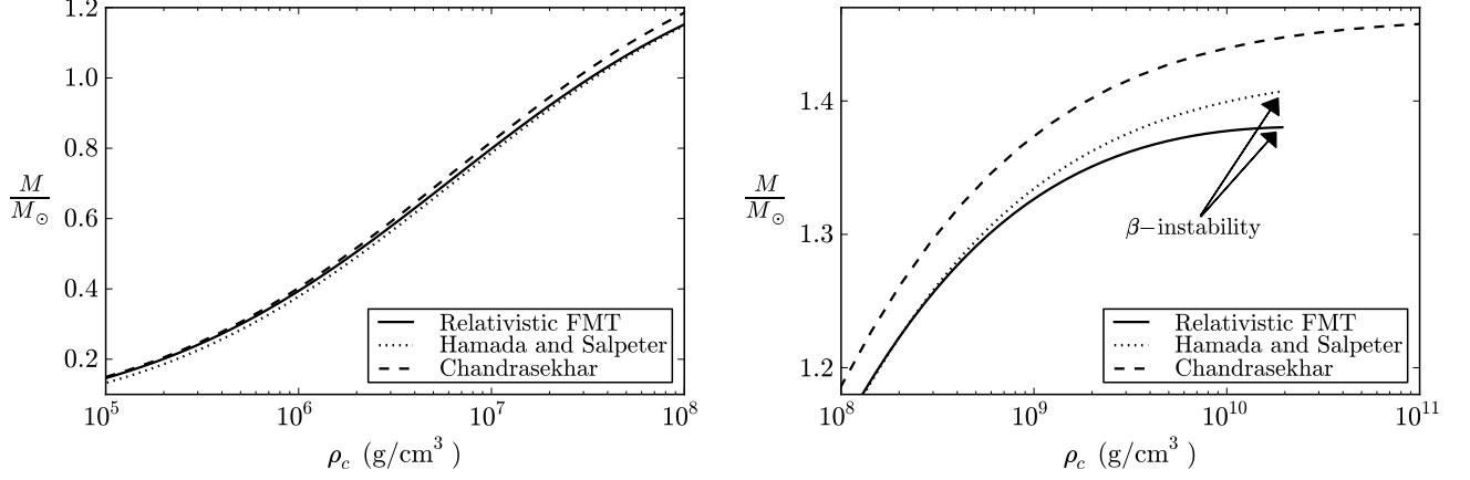
FIG. 7: Mass in solar masses as a function of the central density in the range (left panel) 10^5 – 10^8 \text{g}/\text{cm}^3 and in the range (right panel) 10^8 – 10^{11} \text{g}/\text{cm}^3 for ^{16}\text{O} white dwarfs. The solid curve corresponds to the present work, the dotted curves are the Newtonian configurations of Hamada and Salpeter and the dashed curve are the Newtonian configurations of Chandrasekhar.
