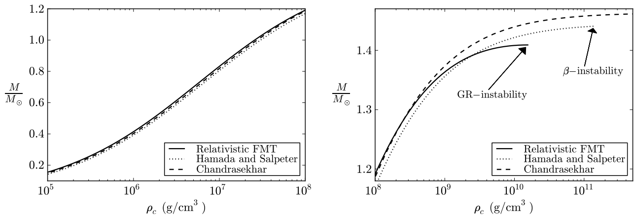
FIG. 3: Mass in solar masses as a function of the central density in the range (left panel) 10^5 – 10^8 \text{g/cm}^3 and in the range (right panel) 10^8 – 5 \times 10^{11} \text{g/cm}^3 for ^4\text{He} white dwarfs. The solid curve corresponds to the present work, the dotted curves are the Newtonian configurations of Hamada and Salpeter and the dashed curve are the Newtonian configurations of Chandrasekhar.
