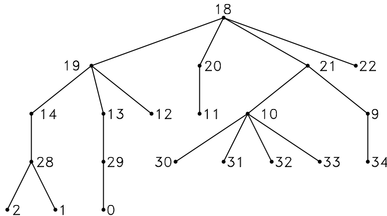
Figure 2: RRG labelling of a tree using Theorem 1 construction
