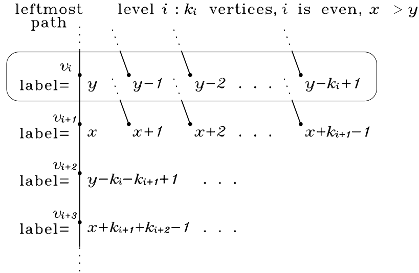
Figure 1: Construction for Theorem 1
