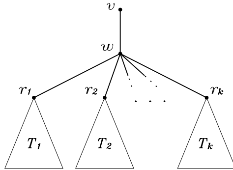
Figure 4: The degree of v is 1
