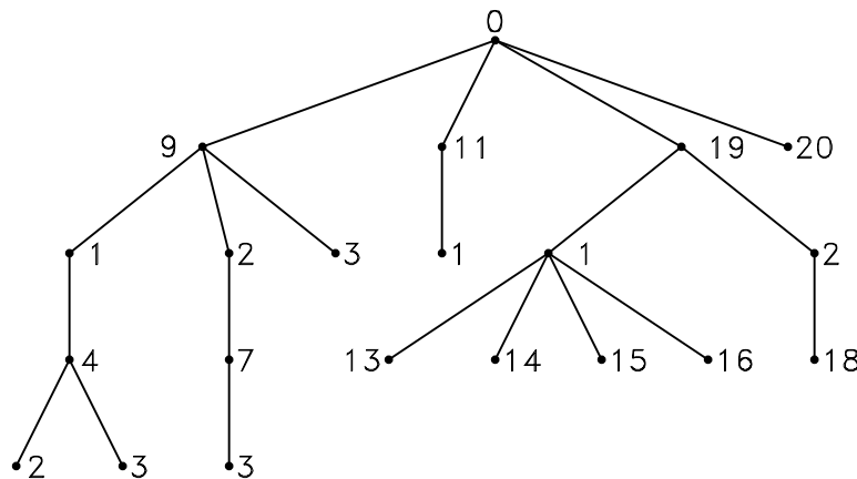
Figure 5: VRG labelling of a tree using construction from Claim 4
