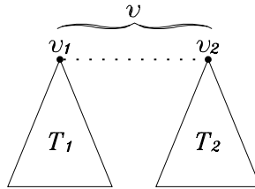
Figure 3: The degree of v is at least 2
