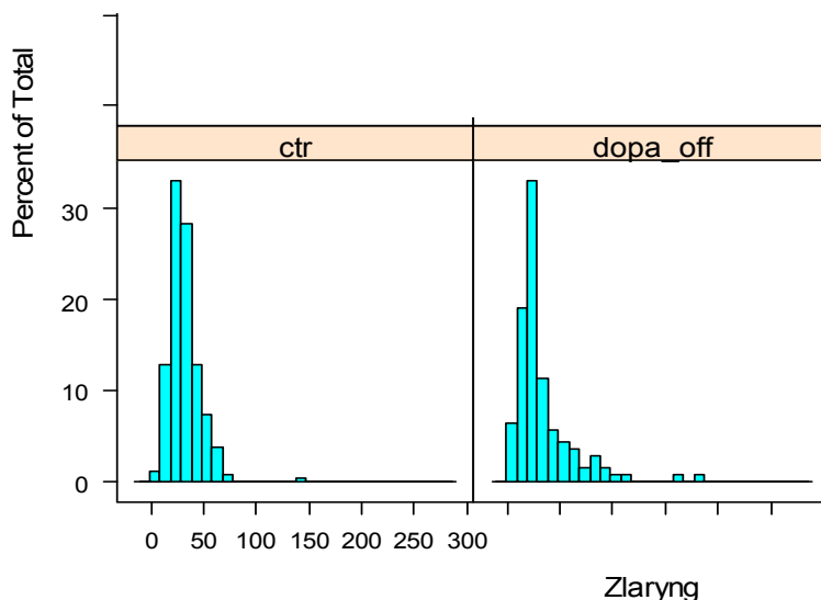
Fig. 10. Histogram of the distribution of values of laryngeal resistance ( Z_{laryng} ). There is a fairly symmetrical distribution for control subjects, while values distributions are more skewed in OFF DOPA patients.
