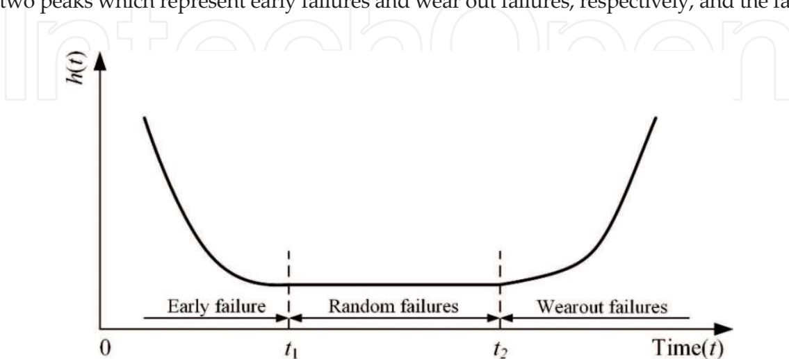
Figure 12. Bathtub curve of failure rates for repairable system.
