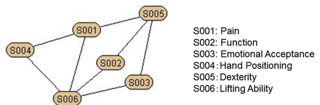
Fig. 1 The AIC network of the MSTS scoring system showed that "pain," and "dexterity," were related to three, and "lifting ability" was related to four other items, indicating these three items had a central role among the six factors of the system.
