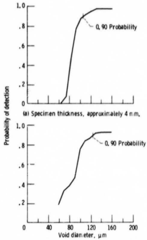
(a) Specimen thickness, approximately 4 mm.
