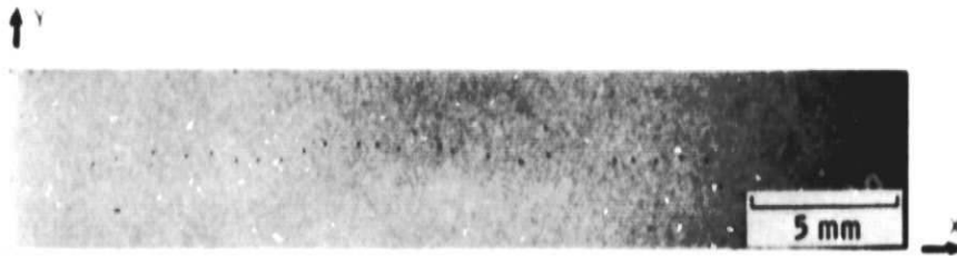
Figure 3. - Optical photograph of as-fired silicon nitride test specimen surface showing location of seeded surface voids along longitudinal (x) axis.
